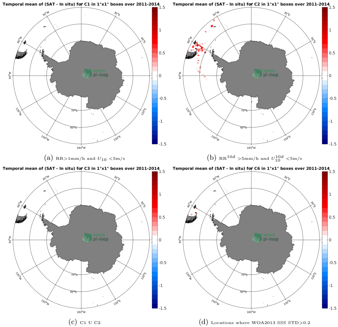
Figure 12: Temporal mean gridded over spatial boxes of size 1^\circ \times 1^\circ of \Delta SSS (Aquarius-L3-JPL-V5-7DAY-RUNNING - TSG-SAMOS) for 4 different subdatasets corresponding to: RR > 1mm/h and U_{10} < 5\text{m/s} (a), RR^{10d} > 5\text{mm/h} and U_{10}^{10d} < 5\text{m/s} (b), C1 U C2 (c), Locations where WOA2013 SSS STD > 0.2 (d).
