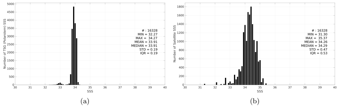
Figure 3: Histograms of SSS from TSG (Polarstern) (a) and Aquarius SSS L3 CAP v5 - 7-Day running (JPL) (b) considering all match-up pairs per bins of 0.1 over the Southern Ocean Pi-MEP region and for the full satellite product period.
