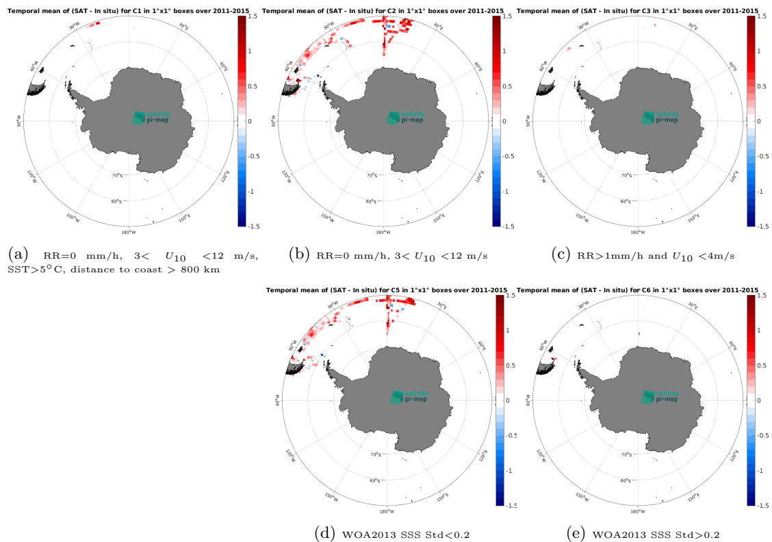
Figure 14: Temporal mean gridded over spatial boxes of size 1^\circ \times 1^\circ of \Delta\text{SSS} (Aquarius SSS L3 CAP v5 - 7-Day running (JPL) - TSG (Polarstern)) for 5 different subdatasets corresponding to:RR=0 mm/h, 3 < U_{10} < 12 m/s, SST>5°C, distance to coast > 800 km (a), RR=0 mm/h, 3 < U_{10} < 12 m/s (b), RR>1mm/h and U_{10} < 4 m/s (c), WOA2013 SSS Std<0.2 (d), WOA2013 SSS Std>0.2 (e).
