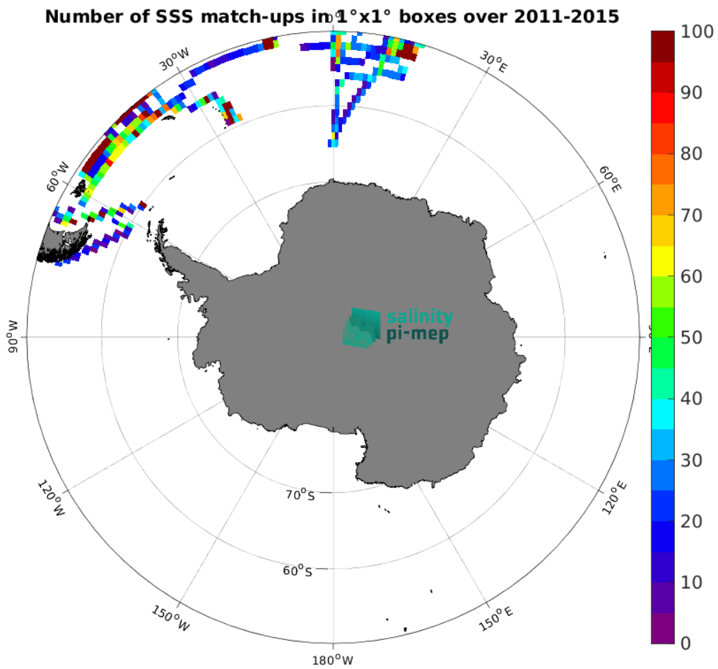
Figure 5: Number of SSS match-ups between TSG (Polarstern) SSS and the Aquarius SSS L3 CAP v5 - 7-Day running (JPL) SSS product for the Southern Ocean Pi-MEP region over 1^\circ \times 1^\circ boxes and for the full satellite product period.
