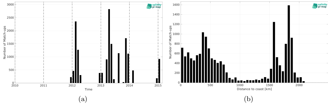
Figure 2: Number of match-ups between TSG (Polarstern) and Aquarius SSS L3 CAP v5 - 7-Day running (JPL) SSS as a function of time (a) and as function of the distance to coast (b) over the Southern Ocean Pi-MEP region and for the full satellite product period.
