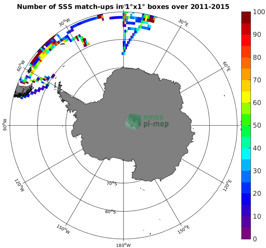
Figure 4: Number of SSS match-ups between TSG-POLARSTERN SSS and the Aquarius-L3-JPL-V5-7DAY-RUNNING SSS product for the Southern Ocean Pi-MEP region over 1^\circ \times 1^\circ boxes and for the full satellite product period.
