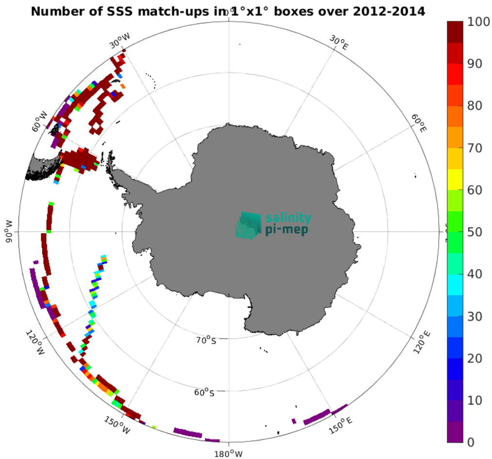
Figure 5: Number of SSS match-ups between TSG (GOSUD-Sailing-ship) SSS and the Aquarius SSS L3 CAP v5 - 7-Day running (JPL) SSS product for the Southern Ocean Pi-MEP region over 1^\circ \times 1^\circ boxes and for the full satellite product period.
