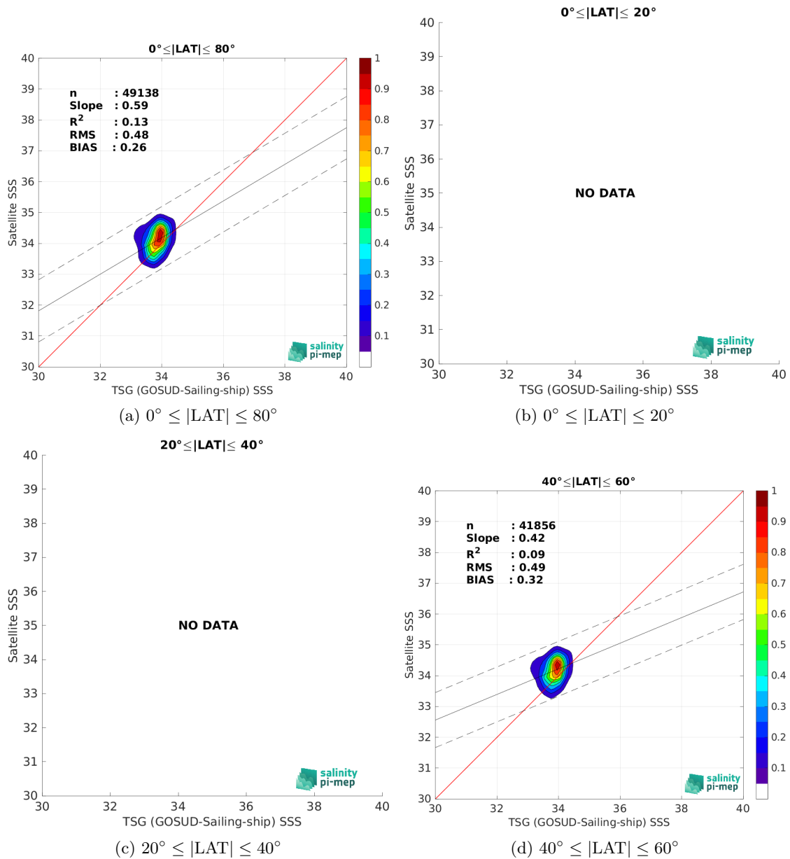
Figure 10: Contour maps of the concentration of Aquarius SSS L3 CAP v5 - 7-Day running (JPL) SSS (y-axis) versus TSG (GOSUD-Sailing-ship) SSS (x-axis) at match-up pairs for different latitude bands. For each plot, the red line shows x=y . The black thin and dashed lines indicate a linear fit through the data cloud and the \pm 95\% confidence levels, respectively. The number match-up pairs n , the slope and R^2 coefficient of the linear fit, the root mean square (RMS) and the mean bias between satellite and in situ data are indicated for each latitude band in each plots.
