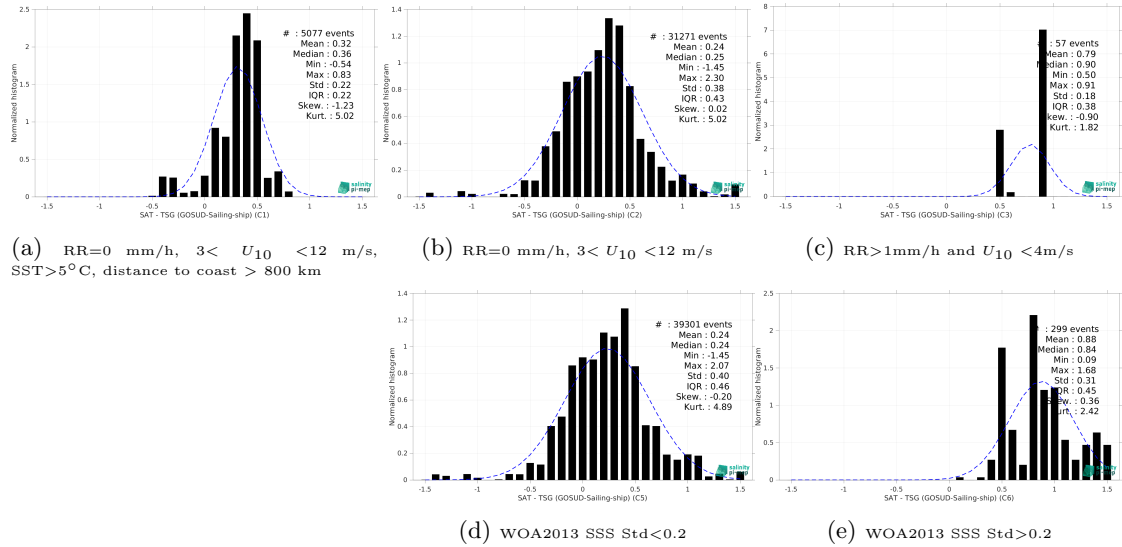
Figure 15: Normalized histogram of \Delta\text{SSS} (Aquarius SSS L3 CAP v5 - 7-Day running (JPL) - TSG (GOSUD-Sailing-ship)) for 5 different subdatasets corresponding to: RR=0 mm/h, 3 < U_{10} < 12 m/s, SST > 5^\circ\text{C} , distance to coast > 800 km (a), RR=0 mm/h, 3 < U_{10} < 12 m/s (b), RR > 1\text{mm/h} and U_{10} < 4\text{m/s} (c), WOA2013 SSS Std < 0.2 (d), WOA2013 SSS Std > 0.2 (e).
