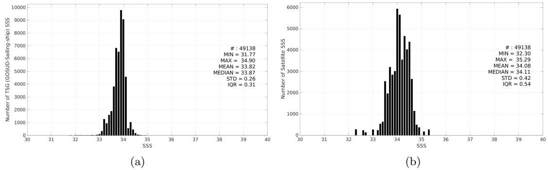
Figure 3: Histograms of SSS from TSG (GOSUD-Sailing-ship) (a) and Aquarius SSS L3 CAP v5 - 7-Day running (JPL) (b) considering all match-up pairs per bins of 0.1 over the Southern Ocean Pi-MEP region and for the full satellite product period.
