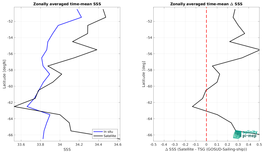
Figure 9: Left panel: Zonal mean SSS from Aquarius SSS L3 CAP v5 - 7-Day running (JPL) satellite product (black) and from TSG (GOSUD-Sailing-ship) (blue). Right panel: Zonal mean of \Delta SSS (Satellite - TSG (GOSUD-Sailing-ship)) for all the collected Pi-MEP match-up pairs estimated over the full satellite product period.
