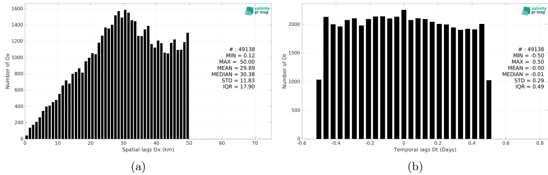
Figure 6: Histograms of the spatial (a) and temporal (b) lags between the location/time of the TSG (GOSUD-Sailing-ship) measurement and the date of the corresponding Aquarius SSS L3 CAP v5 - 7-Day running (JPL) SSS pixel.
