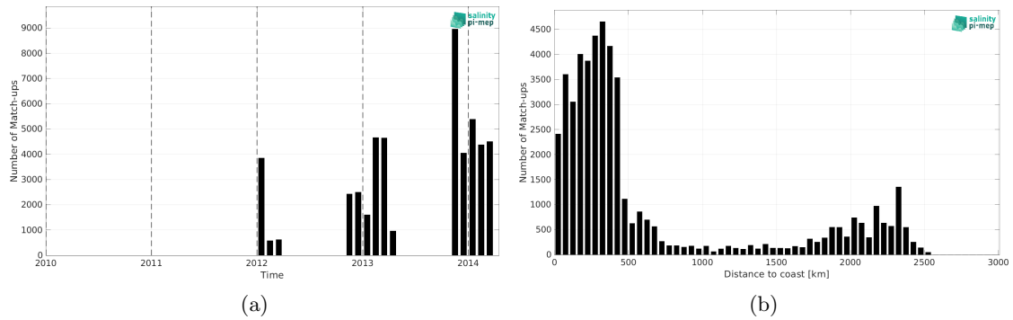
Figure 2: Number of match-ups between TSG (GOSUD-Sailing-ship) and Aquarius SSS L3 CAP v5 - 7-Day running (JPL) SSS as a function of time (a) and as function of the distance to coast (b) over the Southern Ocean Pi-MEP region and for the full satellite product period.
