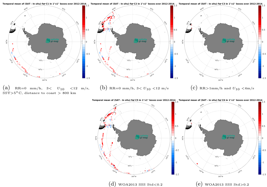
Figure 14: Temporal mean gridded over spatial boxes of size 1^\circ \times 1^\circ of \Delta SSS (Aquarius SSS L3 CAP v5 - 7-Day running (JPL) - TSG (GOSUD-Sailing-ship)) for 5 different subdatasets corresponding to:RR=0 mm/h, 3 < U_{10} < 12 m/s, SST>5°C, distance to coast > 800 km (a), RR=0 mm/h, 3 < U_{10} < 12 m/s (b), RR>1mm/h and U_{10} < 4 m/s (c), WOA2013 SSS Std<0.2 (d), WOA2013 SSS Std>0.2 (e).
