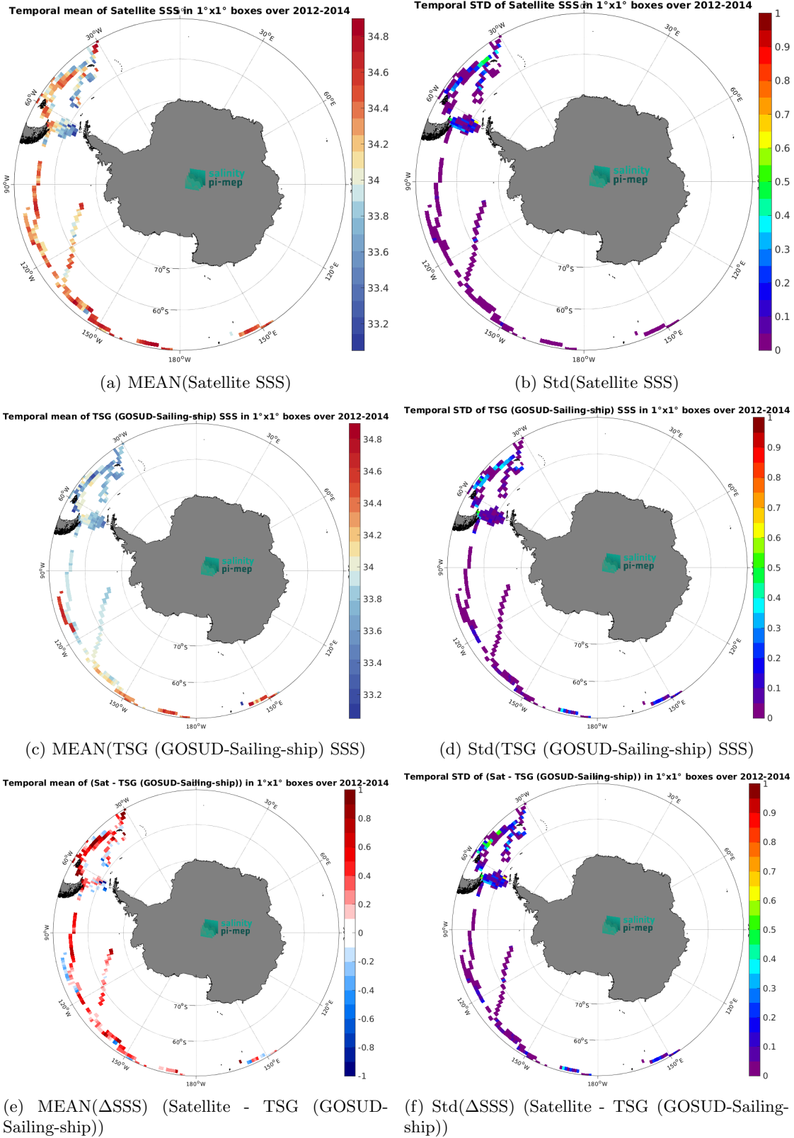
Figure 7: Temporal mean (left) and Std (right) of SSS from Aquarius SSS L3 CAP v5 - 7-Day running (JPL) (top), TSG (GOSUD-Sailing-ship) (middle), and of \Delta SSS (Satellite - TSG (GOSUD-Sailing-ship)). Only match-up pairs are used to generate these maps.
