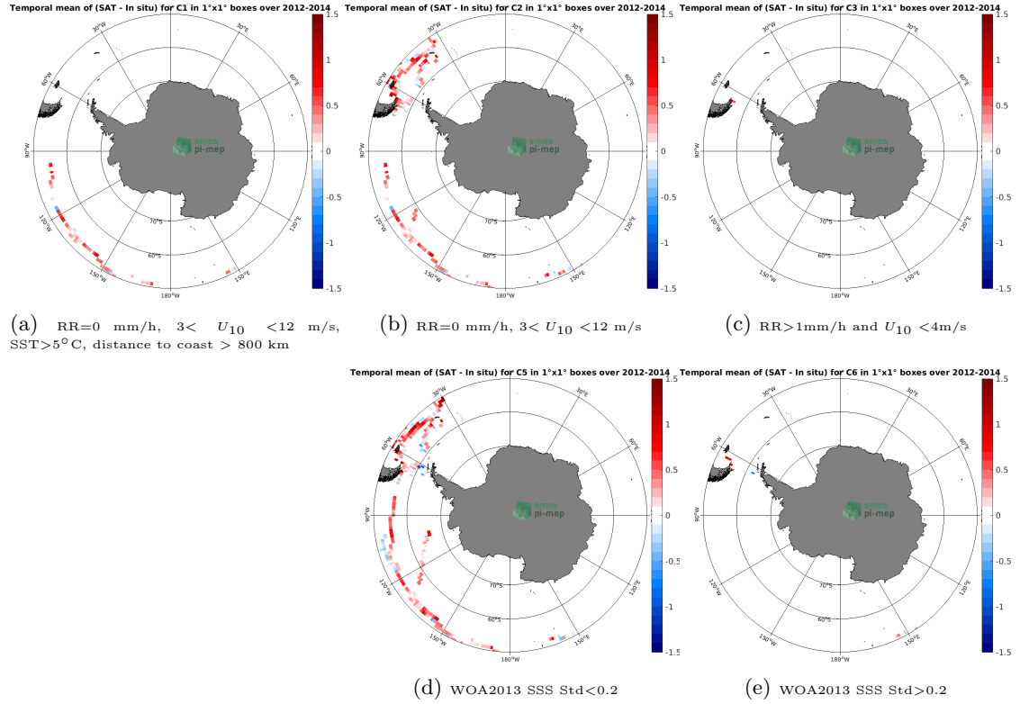
Figure 12: Temporal mean gridded over spatial boxes of size 1°x1° of \Delta\text{SSS} (Aquarius SSS L3 CAP v5 - 7-Day running (JPL) - TSG (GOSUD-Sailing-ship)) for 5 different subdatasets corresponding to: RR=0 mm/h, 3 < U_{10} < 12 m/s, SST > 5^\circ\text{C} , distance to coast > 800 km (a), RR=0 mm/h, 3 < U_{10} < 12 m/s (b), RR > 1 mm/h and U_{10} < 4 m/s (c), WOA2013 SSS Std < 0.2 (d), WOA2013 SSS Std > 0.2 (e).
