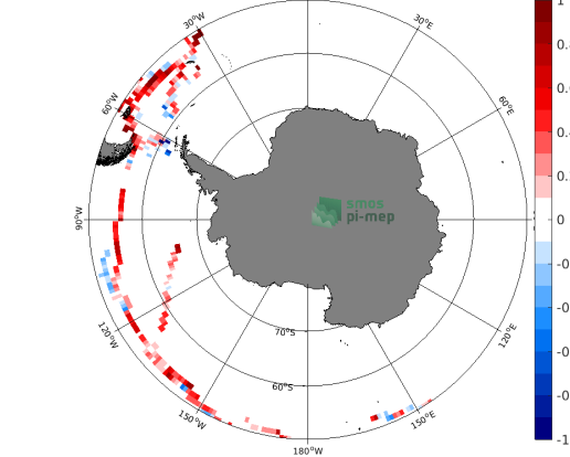
(e) MEAN( \Delta SSS) (Satellite - TSG (GOSUD-Sailing-ship))
