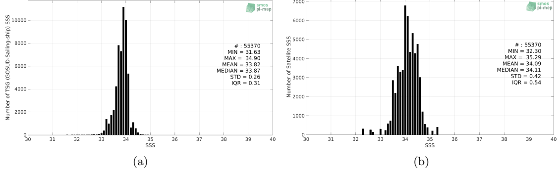
Figure 2: Histograms of SSS from TSG (GOSUD-Sailing-ship) (a) and Aquarius SSS L3 CAP v5 - 7-Day running (JPL) (b) considering all match-up pairs per bins of 0.1 over the Southern Ocean Pi-MEP region and for the full satellite product period.
