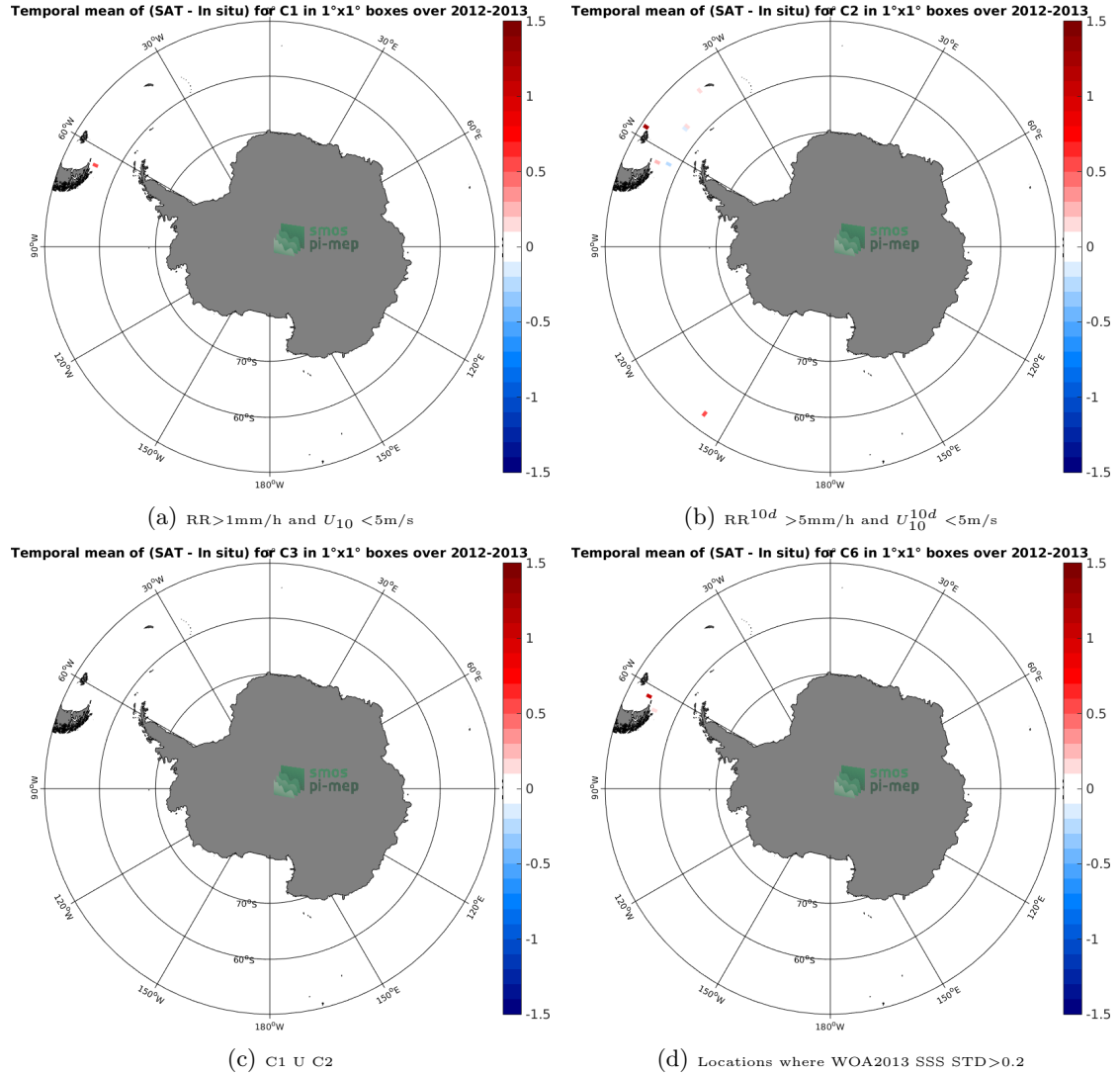
Figure 12: Temporal mean gridded over spatial boxes of size 1^\circ \times 1^\circ of \Delta SSS (Aquarius-L3-JPL-V5-7DAY-RUNNING - TSG-GOSUD-Sailing-ship) for 4 different subdatasets corresponding to: RR > 1\text{mm/h} and U_{10} < 5\text{m/s} (a), RR^{10d} > 5\text{mm/h} and U_{10}^{10d} < 5\text{m/s} (b), C1 U C2 (c), Locations where WOA2013 SSS STD > 0.2 (d).
