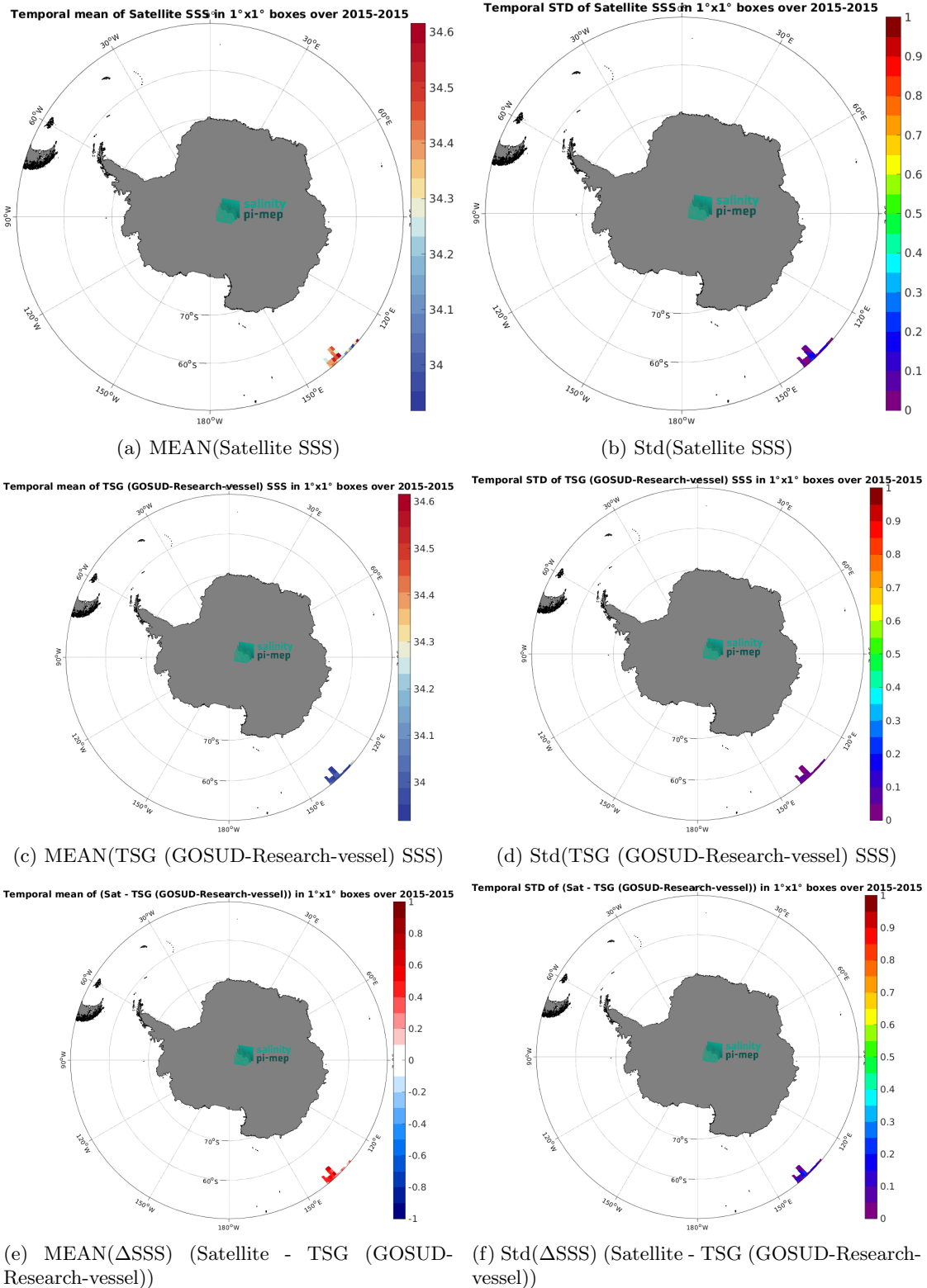
Figure 7: Temporal mean (left) and Std (right) of SSS from Aquarius SSS L3 CAP v5 - 7-Day running (JPL) (top), TSG (GOSUD-Research-vessel) (middle), and of \Delta SSS (Satellite - TSG (GOSUD-Research-vessel)). Only match-up pairs are used to generate these maps.
