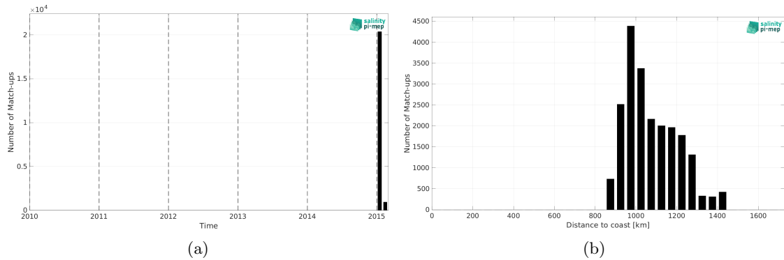
Figure 2: Number of match-ups between TSG (GOSUD-Research-vessel) and Aquarius SSS L3 CAP v5 - 7-Day running (JPL) SSS as a function of time (a) and as function of the distance to coast (b) over the Southern Ocean Pi-MEP region and for the full satellite product period.
