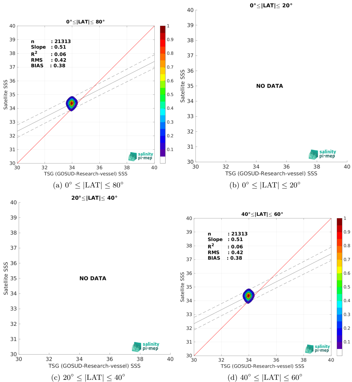
Figure 10: Contour maps of the concentration of Aquarius SSS L3 CAP v5 - 7-Day running (JPL) SSS (y-axis) versus TSG (GOSUD-Research-vessel) SSS (x-axis) at match-up pairs for different latitude bands. For each plot, the red line shows x=y . The black thin and dashed lines indicate a linear fit through the data cloud and the \pm 95\% confidence levels, respectively. The number match-up pairs n , the slope and R^2 coefficient of the linear fit, the root mean square (RMS) and the mean bias between satellite and in situ data are indicated for each latitude band in each plots.
