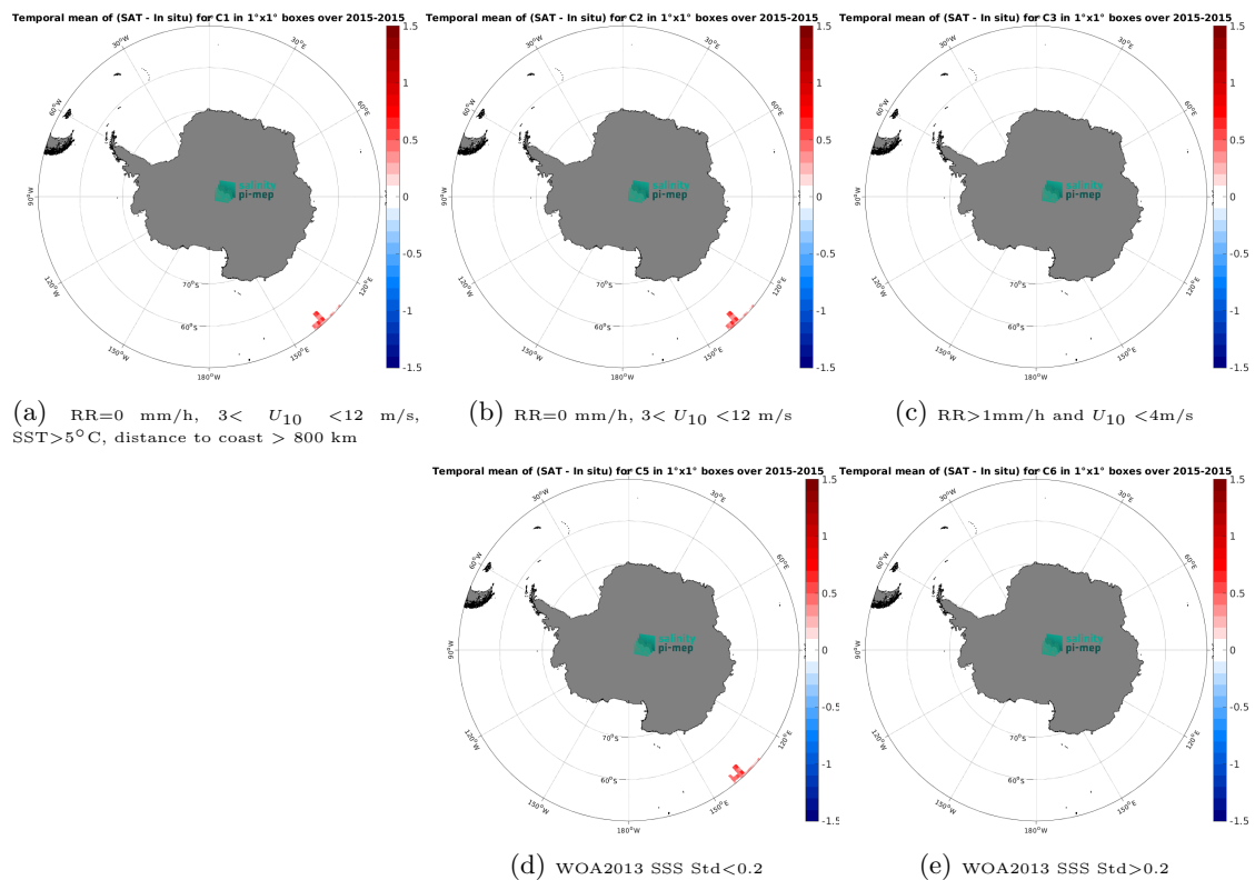
Figure 14: Temporal mean gridded over spatial boxes of size 1^\circ \times 1^\circ of \Delta SSS (Aquarius SSS L3 CAP v5 - 7-Day running (JPL) - TSG (GOSUD-Research-vessel)) for 5 different subdatasets corresponding to:RR=0 mm/h, 3 < U_{10} < 12 m/s, SST >5^\circ\text{C} , distance to coast > 800 km (a), RR=0 mm/h, 3 < U_{10} < 12 m/s (b), RR >1 mm/h and U_{10} < 4 m/s (c), WOA2013 SSS Std <0.2 (d), WOA2013 SSS Std >0.2 (e).
