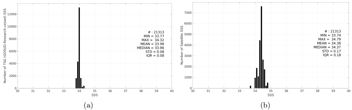
Figure 3: Histograms of SSS from TSG (GOSUD-Research-vessel) (a) and Aquarius SSS L3 CAP v5 - 7-Day running (JPL) (b) considering all match-up pairs per bins of 0.1 over the Southern Ocean Pi-MEP region and for the full satellite product period.
