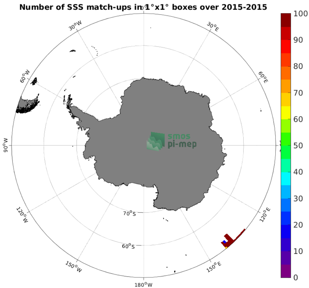
Figure 4: Number of SSS match-ups between TSG (GOSUD-Research-vessel) SSS and the Aquarius SSS L3 CAP v5 - 7-Day running (JPL) SSS product for the Southern Ocean Pi-MEP region over 1^\circ \times 1^\circ boxes and for the full satellite product period.
