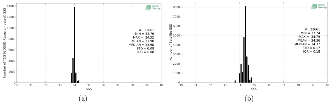
Figure 2: Histograms of SSS from TSG (GOSUD-Research-vessel) (a) and Aquarius SSS L3 CAP v5 - 7-Day running (JPL) (b) considering all match-up pairs per bins of 0.1 over the Southern Ocean Pi-MEP region and for the full satellite product period.
