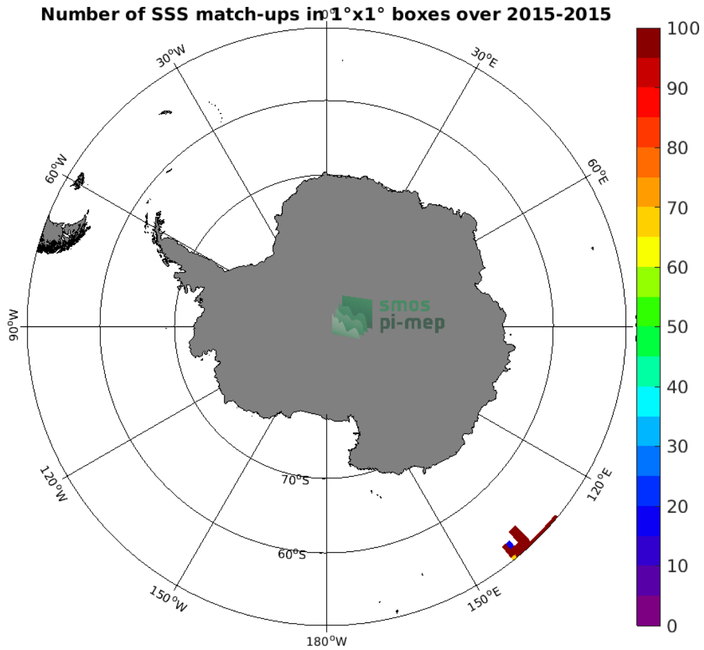
Figure 4: Number of SSS match-ups between TSG (GOSUD-Research-vessel) SSS and the Aquarius SSS L3 CAP v5 - 7-Day running (JPL) SSS product for the Southern Ocean Pi-MEP region over 1^\circ \times 1^\circ boxes and for the full satellite product period.
