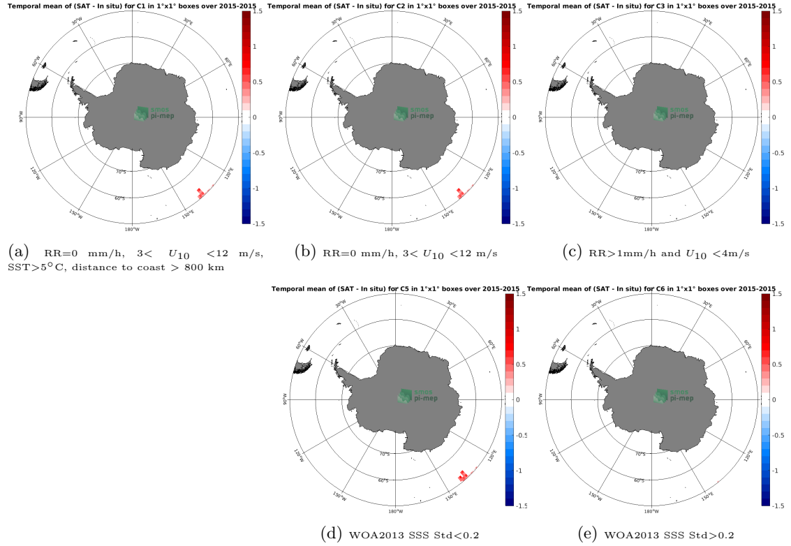
Figure 12: Temporal mean gridded over spatial boxes of size 1^\circ \times 1^\circ of \Delta\text{SSS} (Aquarius SSS L3 CAP v5 - 7-Day running (JPL) - TSG (GOSUD-Research-vessel)) for 5 different subdatasets corresponding to: RR=0 mm/h, 3 < U_{10} < 12 m/s, SST > 5^\circ\text{C} , distance to coast > 800 km (a), RR=0 mm/h, 3 < U_{10} < 12 m/s (b), RR > 1 mm/h and U_{10} < 4 m/s (c), WOA2013 SSS Std < 0.2 (d), WOA2013 SSS Std > 0.2 (e).
