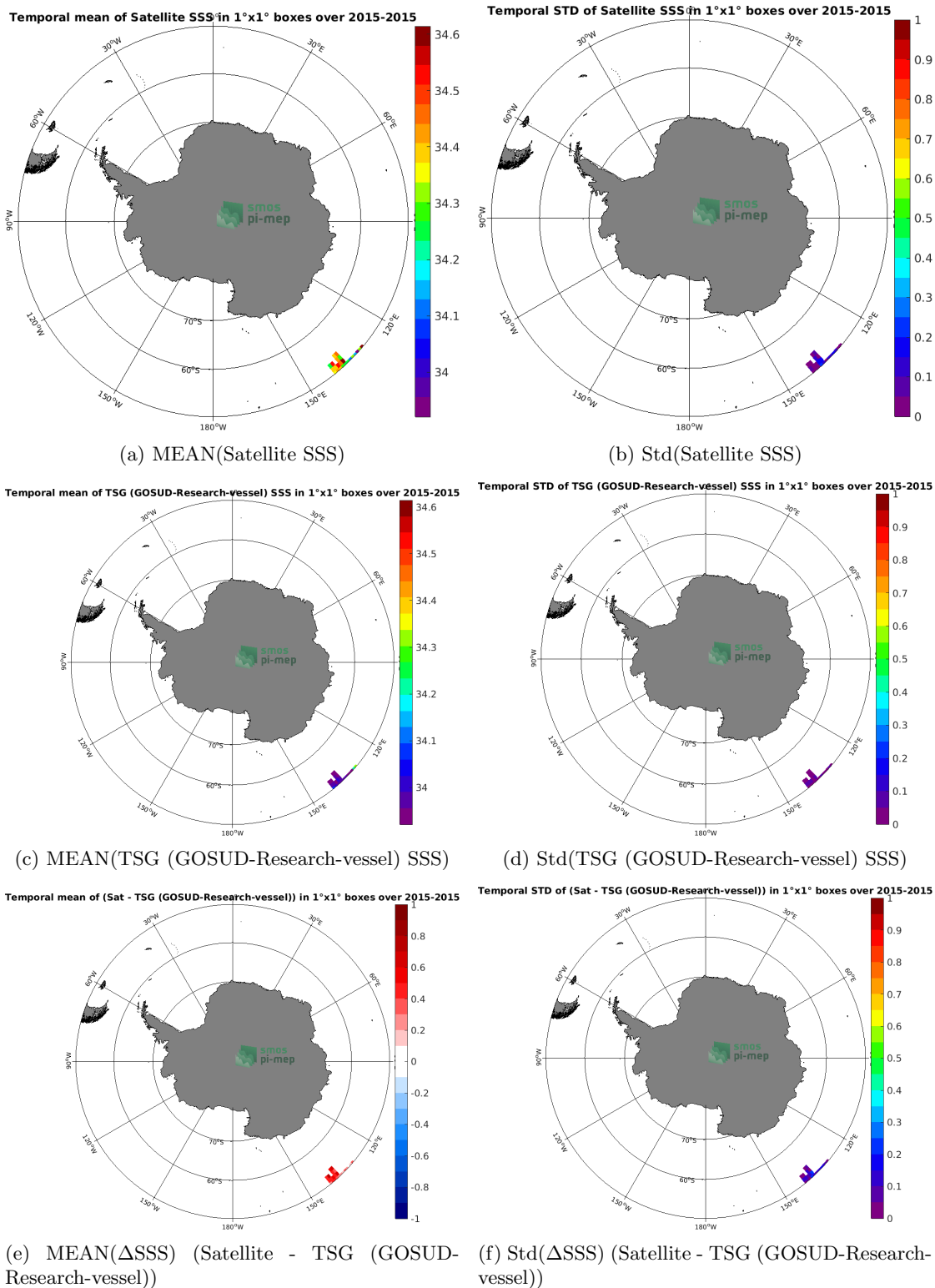
Figure 6: Temporal mean (left) and Std (right) of SSS from Aquarius SSS L3 CAP v5 - 7-Day running (JPL) (top), TSG (GOSUD-Research-vessel) (middle), and of \Delta SSS (Satellite - TSG (GOSUD-Research-vessel)). Only match-up pairs are used to generate these maps.
