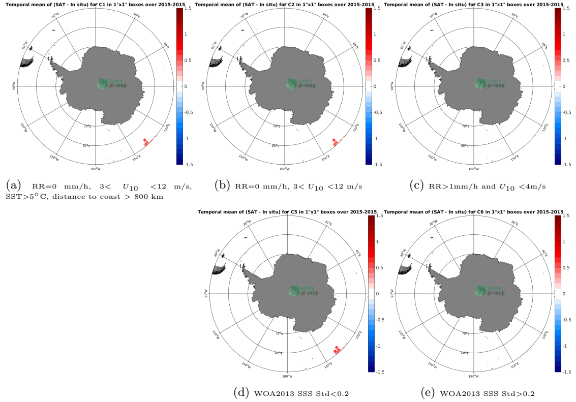
Figure 12: Temporal mean gridded over spatial boxes of size 1°x1° of \Delta\text{SSS} (Aquarius-L3-JPL-V5-7DAY-RUNNING - TSG-GOSUD-Research-vessel) for 5 different subdatasets corresponding to: RR=0 mm/h, 3 < U_{10} < 12 m/s, SST > 5^\circ\text{C} , distance to coast > 800 km (a), RR=0 mm/h, 3 < U_{10} < 12 m/s (b), RR > 1 mm/h and U_{10} < 4 m/s (c), WOA2013 SSS Std < 0.2 (d), WOA2013 SSS Std > 0.2 (e).
