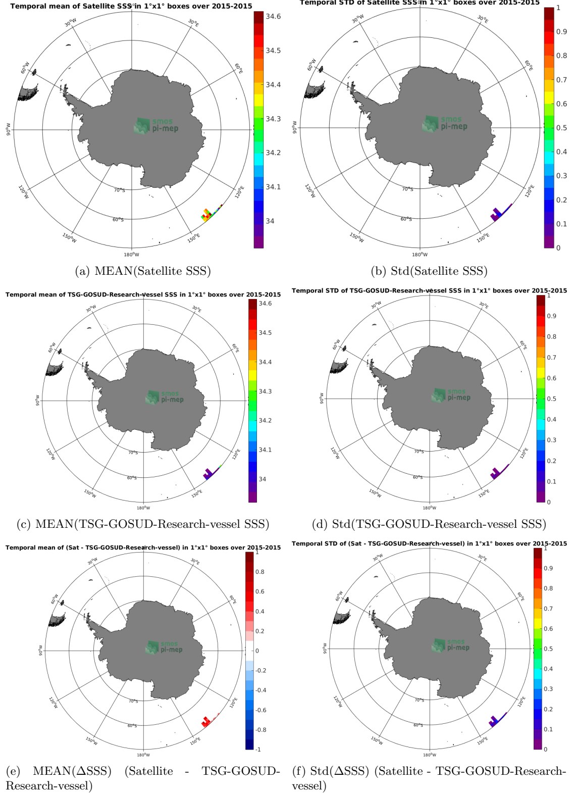
Figure 6: Temporal mean (left) and Std (right) of SSS from Aquarius-L3-JPL-V5-7DAY-RUNNING (top), TSG-GOSUD-Research-vessel (middle), and of \Delta SSS (Satellite - TSG-GOSUD-Research-vessel). Only match-up pairs are used to generate these maps.
