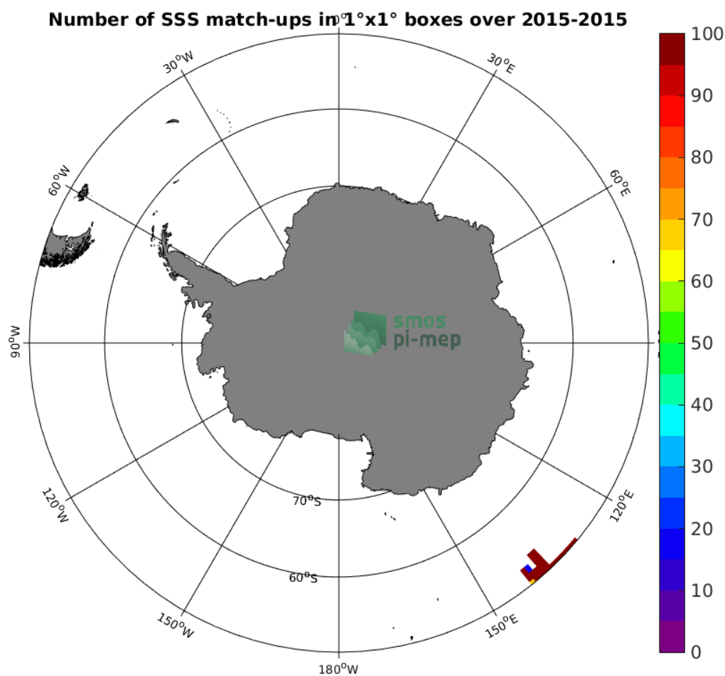
Figure 4: Number of SSS match-ups between TSG-GOSUD-Research-vessel SSS and the Aquarius-L3-JPL-V5-7DAY-RUNNING SSS product for the Southern Ocean Pi-MEP region over 1^\circ \times 1^\circ boxes and for the full satellite product period.
