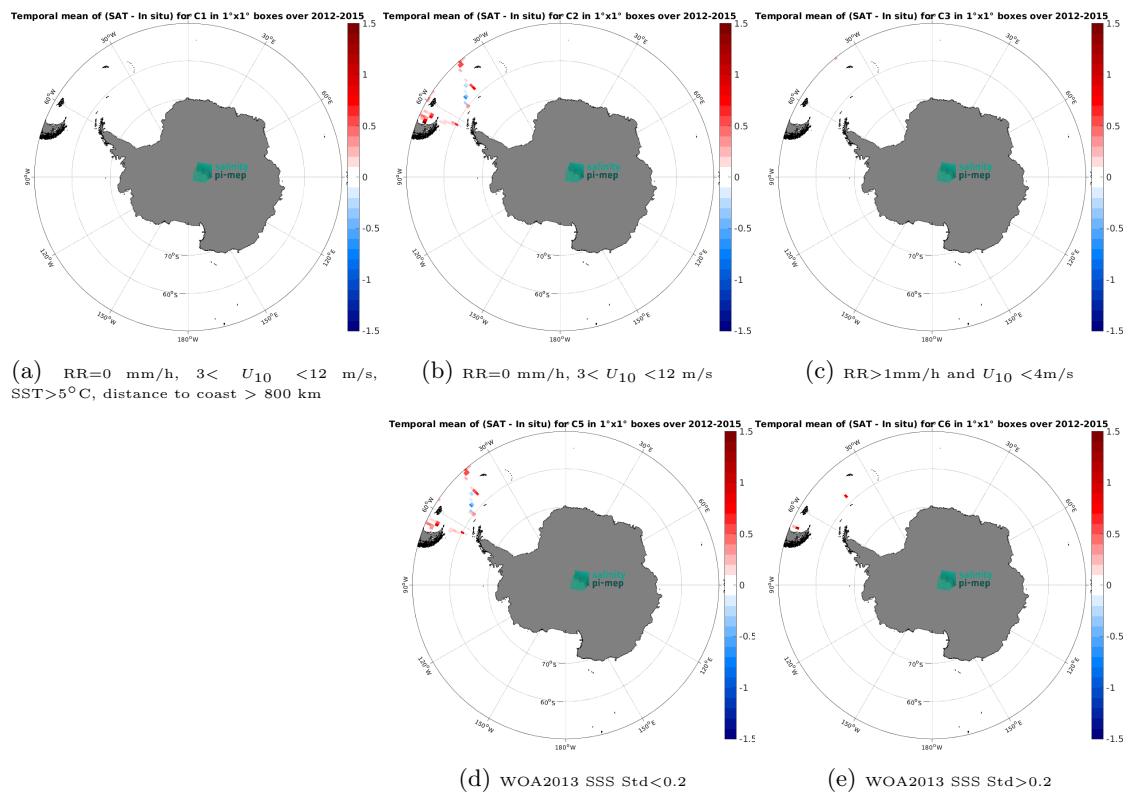
Figure 14: Temporal mean gridded over spatial boxes of size 1^\circ \times 1^\circ of \Delta\text{SSS} (Aquarius SSS L3 CAP v5 - 7-Day running (JPL) - TSG (CSIC-UTM)) for 5 different subdatasets corresponding to:RR=0 mm/h, 3 < U_{10} < 12 m/s, SST>5°C, distance to coast > 800 km (a), RR=0 mm/h, 3 < U_{10} < 12 m/s (b), RR>1mm/h and U_{10} < 4 m/s (c), WOA2013 SSS Std<0.2 (d), WOA2013 SSS Std>0.2 (e).
