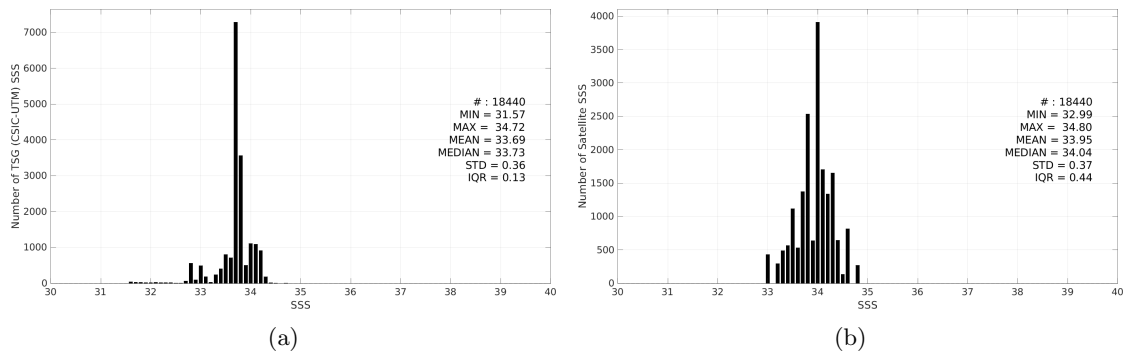
Figure 3: Histograms of SSS from TSG (CSIC-UTM) (a) and Aquarius SSS L3 CAP v5 - 7-Day running (JPL) (b) considering all match-up pairs per bins of 0.1 over the Southern Ocean Pi-MEP region and for the full satellite product period.
