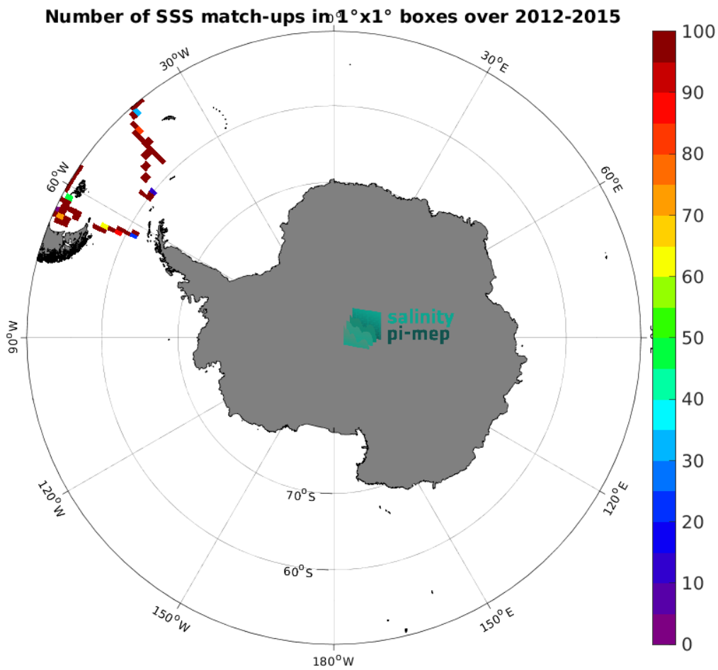
Figure 5: Number of SSS match-ups between TSG (CSIC-UTM) SSS and the Aquarius SSS L3 CAP v5 - 7-Day running (JPL) SSS product for the Southern Ocean Pi-MEP region over 1^{\circ} \times 1^{\circ} boxes and for the full satellite product period.
