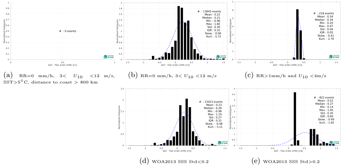
Figure 15: Normalized histogram of \Delta SSS (Aquarius SSS L3 CAP v5 - 7-Day running (JPL) - TSG (CSIC-UTM)) for 5 different subdatasets corresponding to: RR=0 mm/h, 3 < U_{10} < 12 m/s, SST > 5°C, distance to coast > 800 km (a), RR=0 mm/h, 3 < U_{10} < 12 m/s (b), RR > 1mm/h and U_{10} < 4 m/s (c), WOA2013 SSS Std < 0.2 (d), WOA2013 SSS Std > 0.2 (e).
