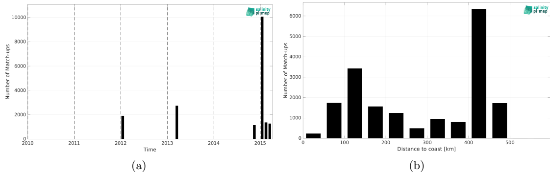
Figure 2: Number of match-ups between TSG (CSIC-UTM) and Aquarius SSS L3 CAP v5 - 7-Day running (JPL) SSS as a function of time (a) and as function of the distance to coast (b) over the Southern Ocean Pi-MEP region and for the full satellite product period.
