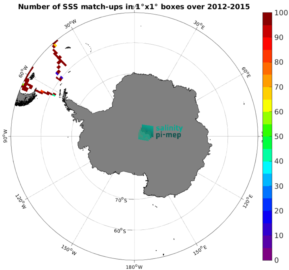
Figure 4: Number of SSS match-ups between TSG (CSIC-UTM) SSS and the Aquarius SSS L3 CAP v5 - 7-Day running (JPL) SSS product for the Southern Ocean Pi-MEP region over 1^{\circ} \times 1^{\circ} boxes and for the full satellite product period.
