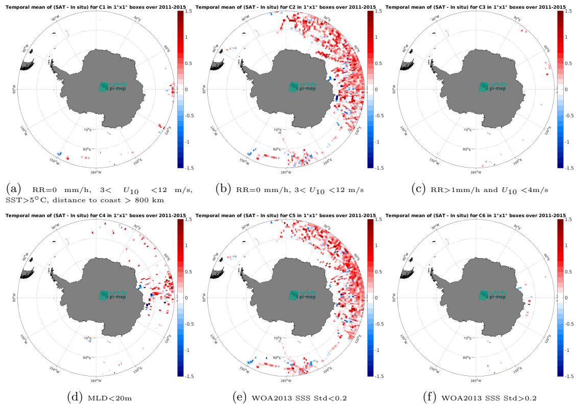
Figure 14: Temporal mean gridded over spatial boxes of size 1^\circ \times 1^\circ of \Delta\text{SSS} (Aquarius SSS L3 CAP v5 - 7-Day running (JPL) - Marine mammals) for 6 different subdatasets corresponding to:RR=0 mm/h, 3 < U_{10} < 12 m/s, SST>5°C, distance to coast > 800 km (a), RR=0 mm/h, 3 < U_{10} < 12 m/s (b), RR>1mm/h and U_{10} < 4 m/s (c),MLD<20m (d),WOA2013 SSS Std<0.2 (e),WOA2013 SSS Std>0.2 (f).
