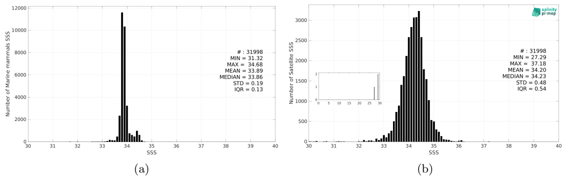
Figure 3: Histograms of SSS from Marine mammals (a) and Aquarius SSS L3 CAP v5 - 7-Day running (JPL) (b) considering all match-up pairs per bins of 0.1 over the Southern Ocean Pi-MEP region and for the full satellite product period.
