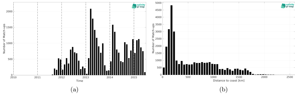
Figure 2: Number of match-ups between Marine mammals and Aquarius SSS L3 CAP v5 - 7-Day running (JPL) SSS as a function of time (a) and as function of the distance to coast (b) over the Southern Ocean Pi-MEP region and for the full satellite product period.
