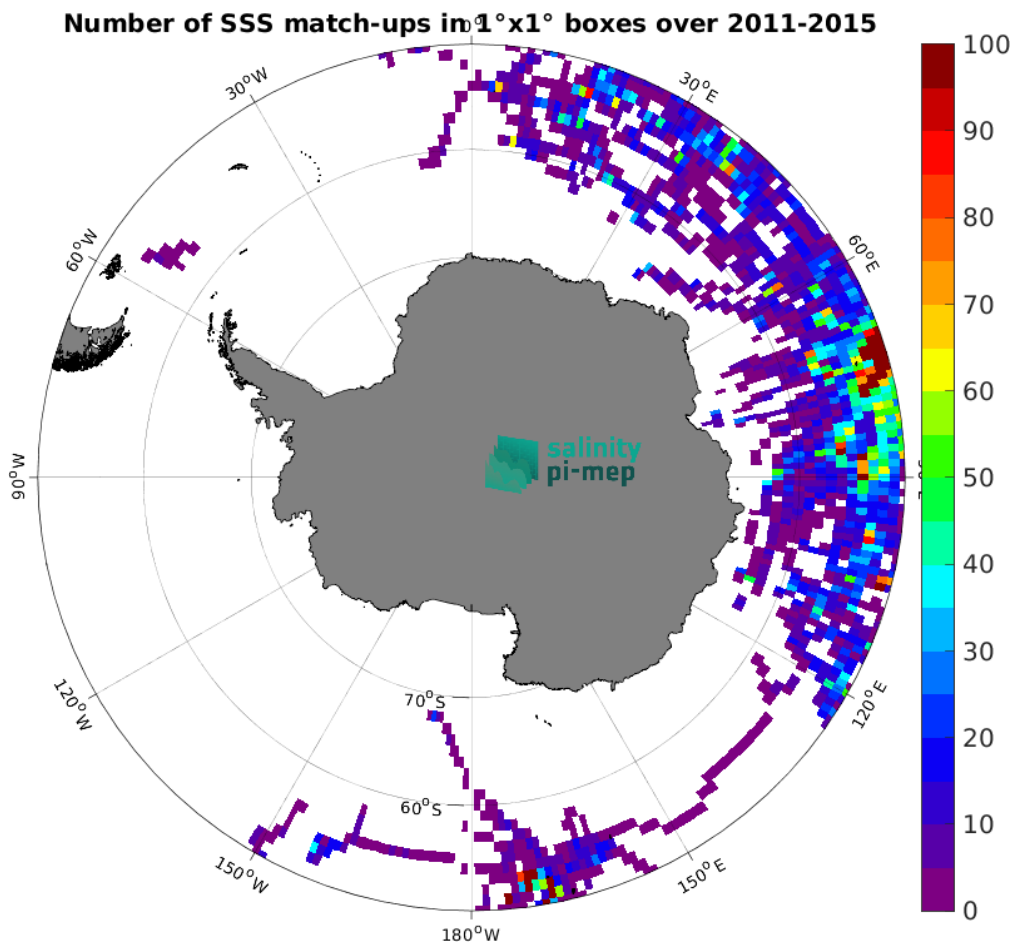
Figure 5: Number of SSS match-ups between Marine mammals SSS and the Aquarius SSS L3 CAP v5 - 7-Day running (JPL) SSS product for the Southern Ocean Pi-MEP region over 1^\circ \times 1^\circ boxes and for the full satellite product period.
