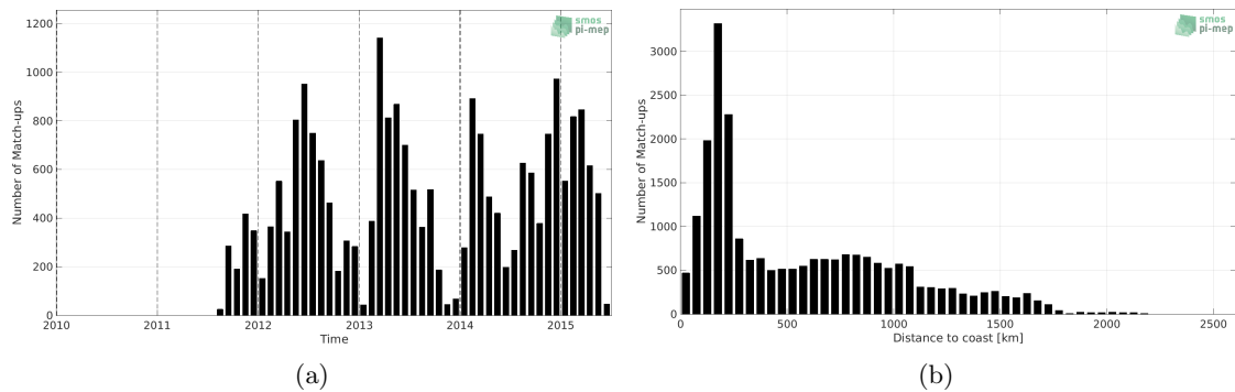
Figure 1: Number of match-ups between Sea mammals and Aquarius SSS L3 CAP v5 - 7-Day running (JPL) SSS as a function of time (a) and as function of the distance to coast (b) over the Southern Ocean Pi-MEP region and for the full satellite product period.
