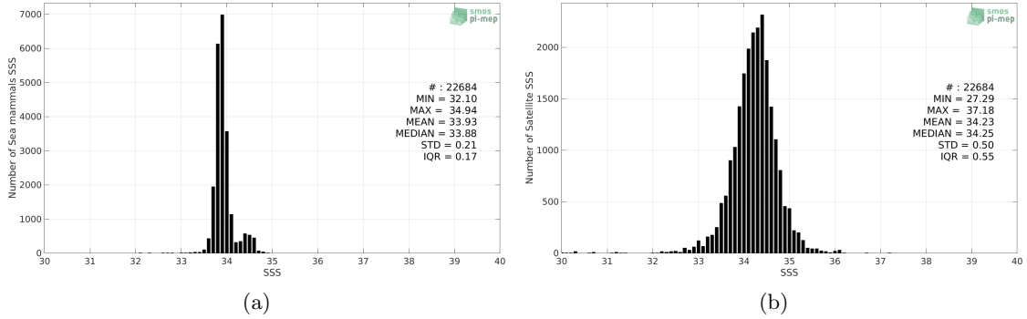
Figure 2: Histograms of SSS from Sea mammals (a) and Aquarius SSS L3 CAP v5 - 7-Day running (JPL) (b) considering all match-up pairs per bins of 0.1 over the Southern Ocean Pi-MEP region and for the full satellite product period.
