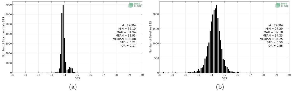
Figure 2: Histograms of SSS from Sea mammals (a) and Aquarius-L3-JPL-V5-7DAY-RUNNING (b) considering all match-up pairs per bins of 0.1 over the Southern Ocean Pi-MEP region and for the full satellite product period.
