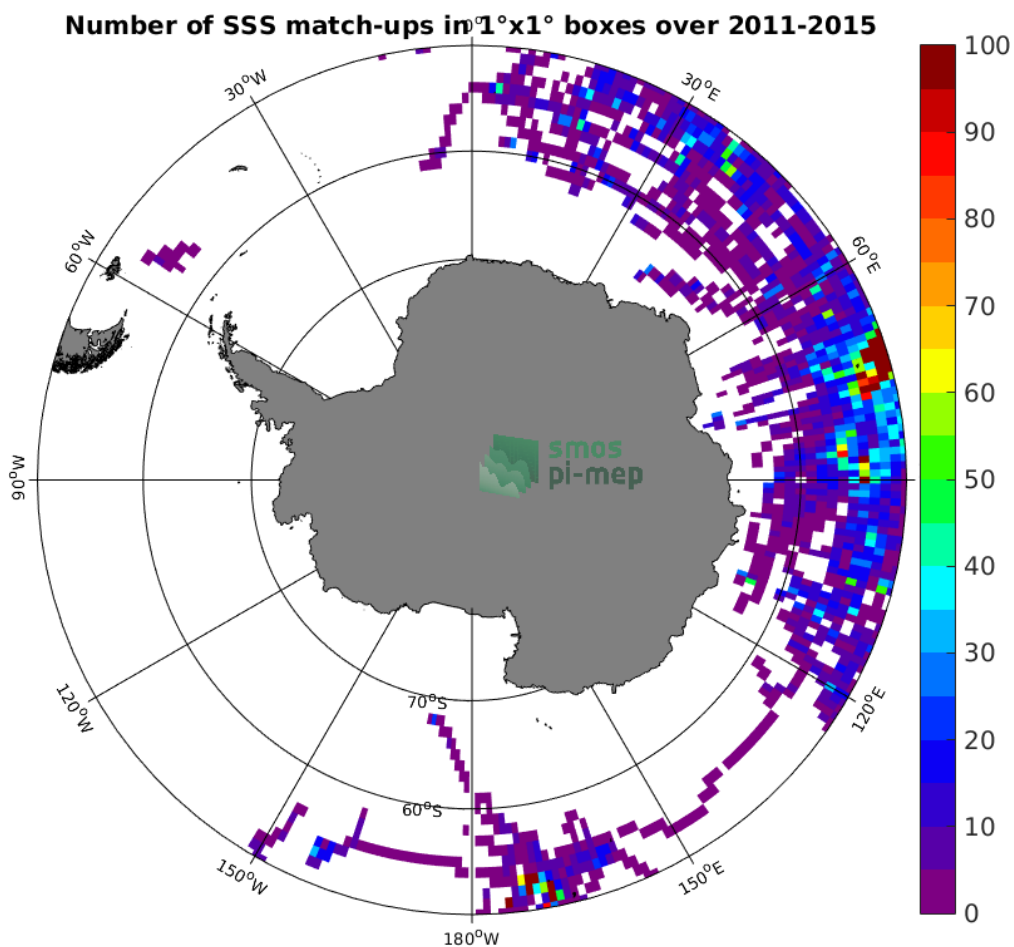
Figure 4: Number of SSS match-ups between Sea mammals SSS and the Aquarius-L3-JPL-V5-7DAY-RUNNING SSS product for the Southern Ocean Pi-MEP region over 1^\circ \times 1^\circ boxes and for the full satellite product period.
