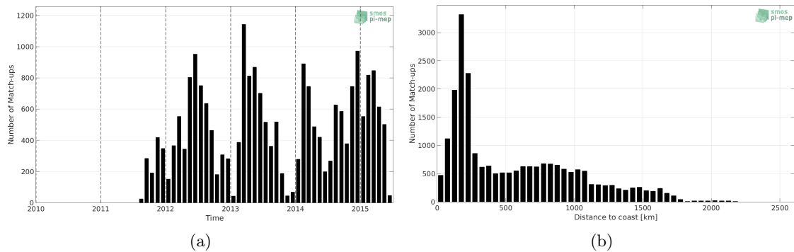
Figure 1: Number of match-ups between Sea mammals and Aquarius-L3-JPL-V5-7DAY-RUNNING SSS as a function of time (a) and as function of the distance to coast (b) over the Southern Ocean Pi-MEP region and for the full satellite product period.
