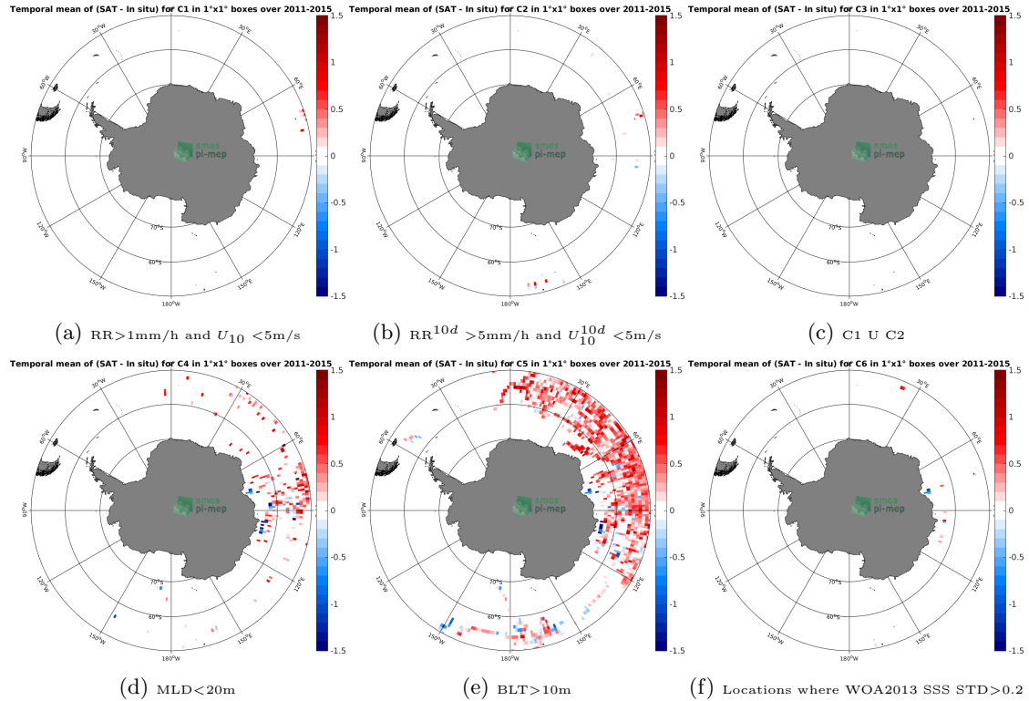
Figure 12: Temporal mean gridded over spatial boxes of size 1^\circ \times 1^\circ of \Delta\text{SSS} (Aquarius-L3-JPL-V5-7DAY-RUNNING - Sea mammals) for 6 different subdatasets corresponding to: RR > 1\text{mm/h} and U_{10} < 5\text{m/s} (a), RR^{10d} > 5\text{mm/h} and U_{10}^{10d} < 5\text{m/s} (b), C1 U C2 (c), \text{MLD} < 20\text{m} (d), \text{BLT} > 10\text{m} (e), Locations where WOA2013 SSS STD > 0.2 (f).
