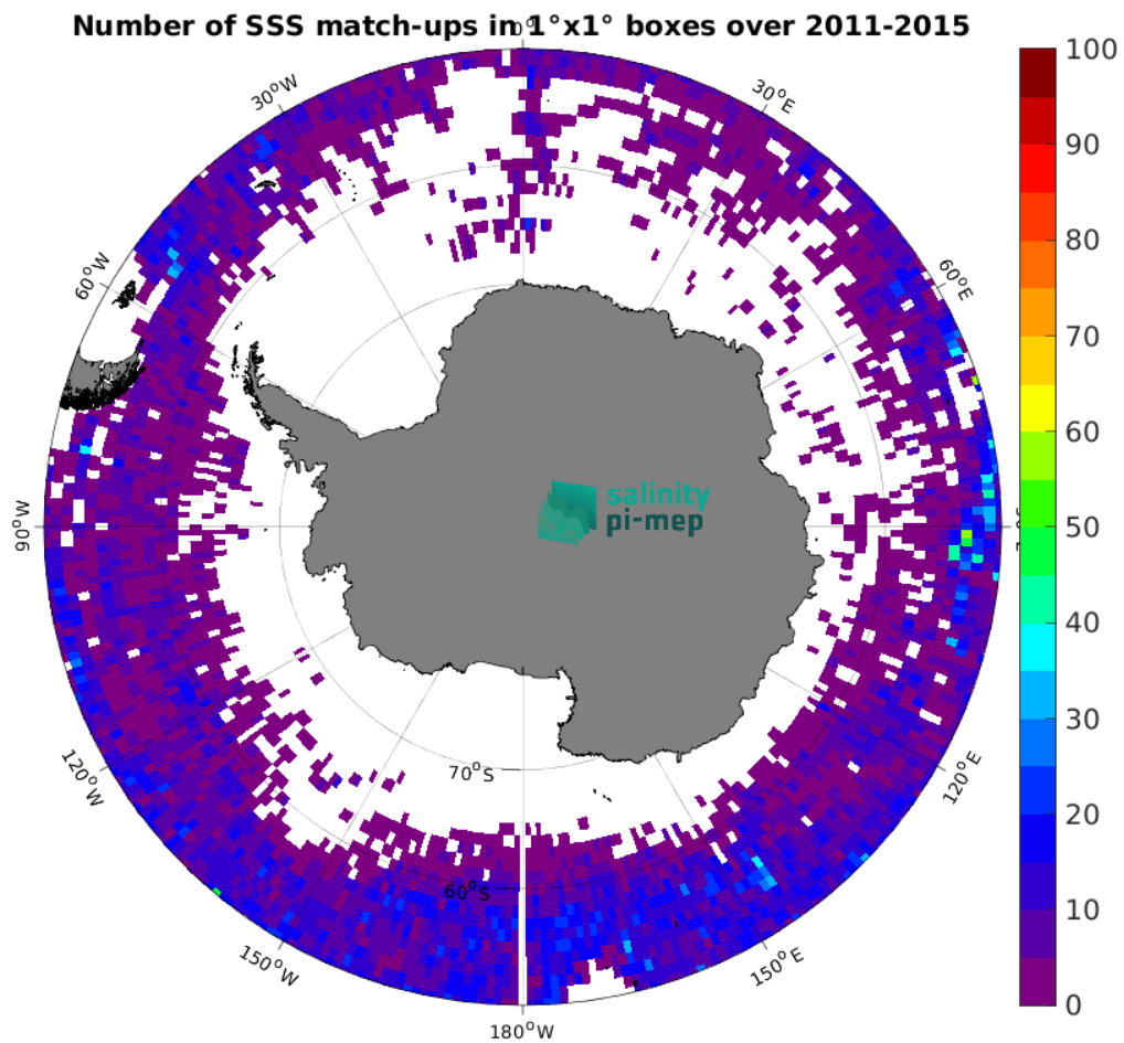
Figure 5: Number of SSS match-ups between Argo SSS and the Aquarius SSS L3 CAP v5 - 7-Day running (JPL) SSS product for the Southern Ocean Pi-MEP region over 1^{\circ} \times 1^{\circ} boxes and for the full satellite product period.
