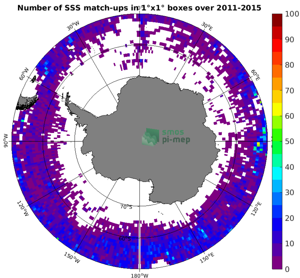
Figure 4: Number of SSS match-ups between Argo SSS and the Aquarius SSS L3 CAP v5 - 7-Day running (JPL) SSS product for the Southern Ocean Pi-MEP region over 1^\circ \times 1^\circ boxes and for the full satellite product period.
