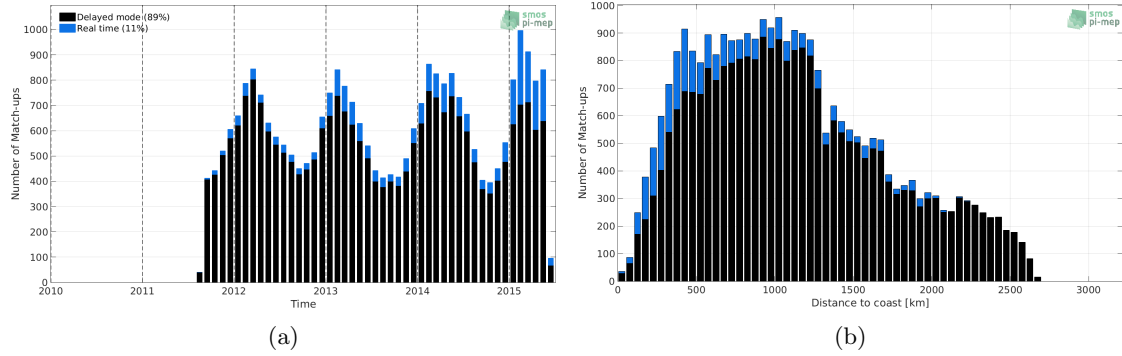
Figure 1: Number of match-ups between Argo and Aquarius-L3-JPL-V5-7DAY-RUNNING SSS as a function of time (a) and as function of the distance to coast (b) over the Southern Ocean Pi-MEP region and for the full satellite product period.
