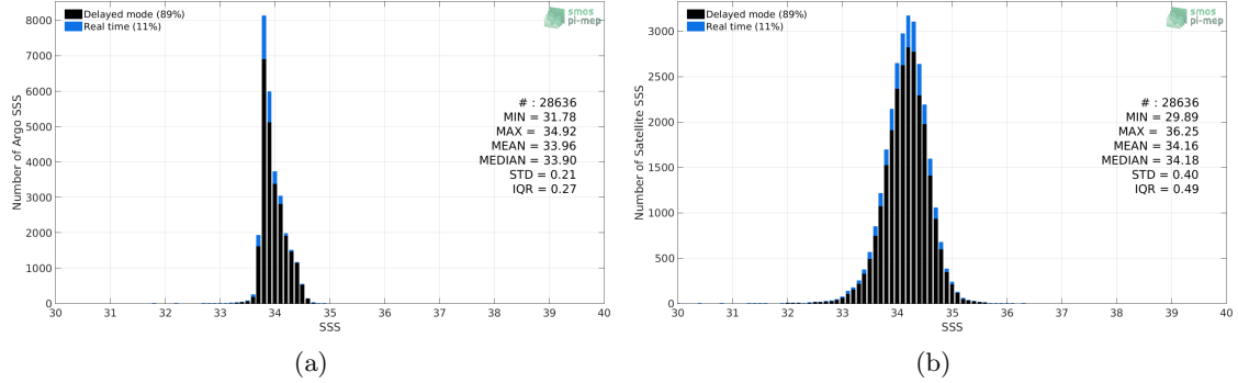
Figure 2: Histograms of SSS from Argo (a) and Aquarius-L3-JPL-V5-7DAY-RUNNING (b) considering all match-up pairs per bins of 0.1 over the Southern Ocean Pi-MEP region and for the full satellite product period.
