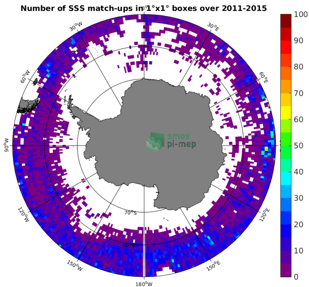
Figure 4: Number of SSS match-ups between Argo SSS and the Aquarius-L3-JPL-V5-7DAY-RUNNING SSS product for the Southern Ocean Pi-MEP region over 1^\circ \times 1^\circ boxes and for the full satellite product period.
