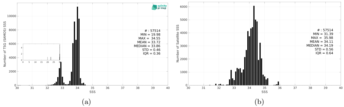
Figure 3: Histograms of SSS from TSG (SAMOS) (a) and Aquarius SSS L3 CAP v5 - Monthly (JPL) (b) considering all match-up pairs per bins of 0.1 over the Southern Ocean Pi-MEP region and for the full satellite product period.
