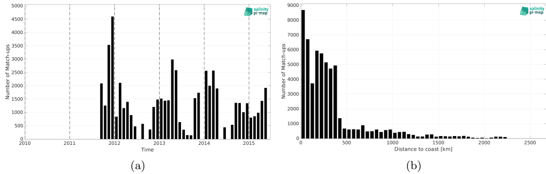
Figure 2: Number of match-ups between TSG (SAMOS) and Aquarius SSS L3 CAP v5 - Monthly (JPL) SSS as a function of time (a) and as function of the distance to coast (b) over the Southern Ocean Pi-MEP region and for the full satellite product period.
