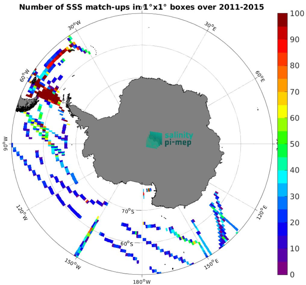
Figure 5: Number of SSS match-ups between TSG (SAMOS) SSS and the Aquarius SSS L3 CAP v5 - Monthly (JPL) SSS product for the Southern Ocean Pi-MEP region over 1^\circ \times 1^\circ boxes and for the full satellite product period.
