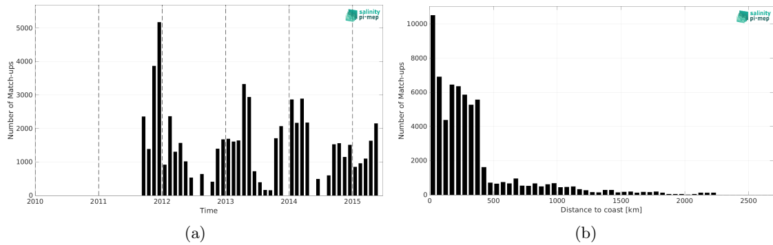
Figure 1: Number of match-ups between TSG (SAMOS) and Aquarius SSS L3 CAP v5 - Monthly (JPL) SSS as a function of time (a) and as function of the distance to coast (b) over the Southern Ocean Pi-MEP region and for the full satellite product period.
