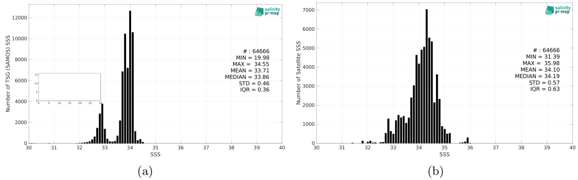
Figure 2: Histograms of SSS from TSG (SAMOS) (a) and Aquarius SSS L3 CAP v5 - Monthly (JPL) (b) considering all match-up pairs per bins of 0.1 over the Southern Ocean Pi-MEP region and for the full satellite product period.
