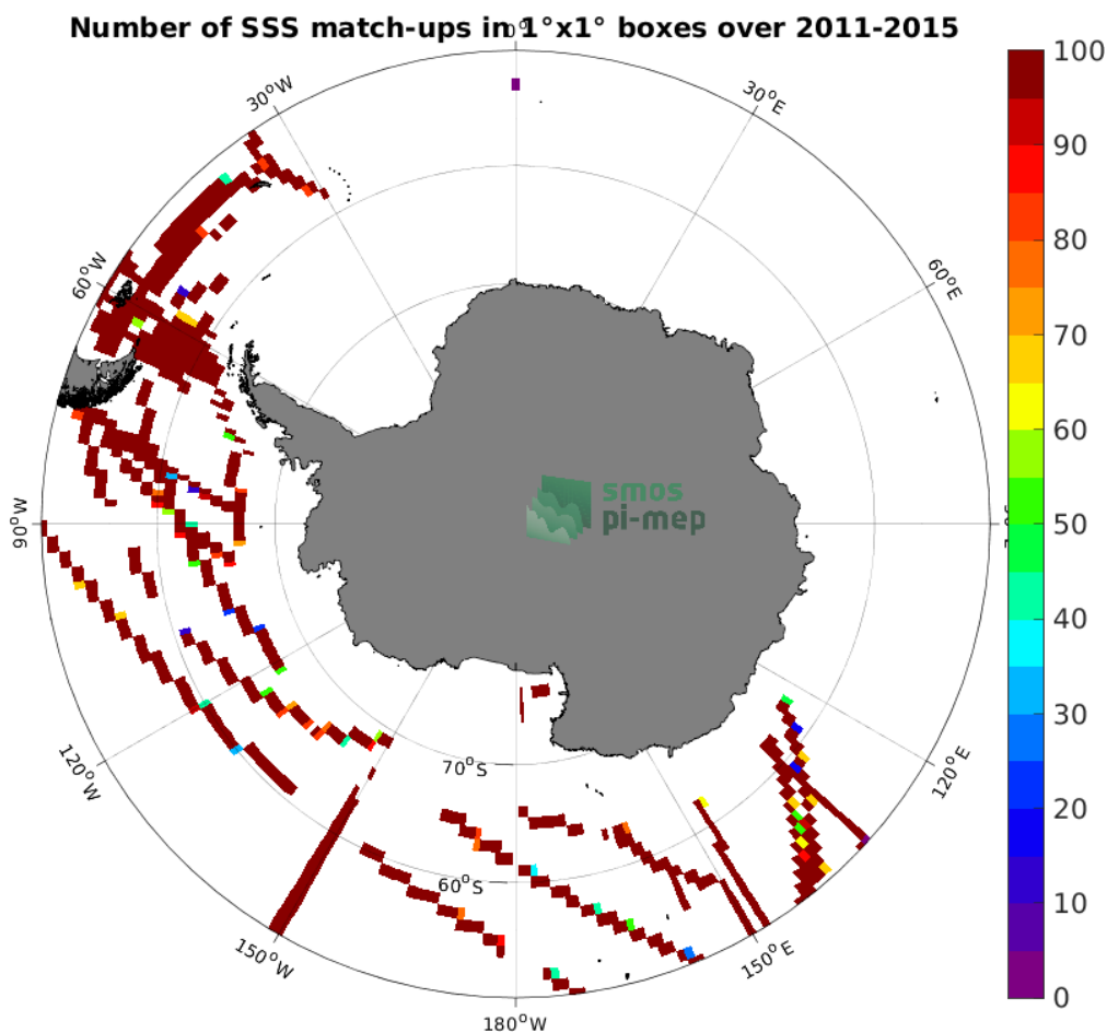
Figure 4: Number of SSS match-ups between TSG (SAMOS) SSS and the Aquarius SSS L3 CAP v5 - Monthly (JPL) SSS product for the Southern Ocean Pi-MEP region over 1^\circ \times 1^\circ boxes and for the full satellite product period.
