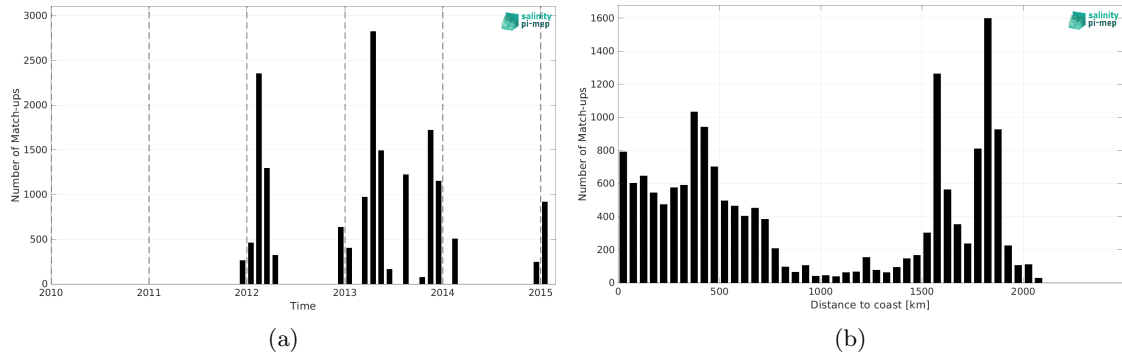
Figure 2: Number of match-ups between TSG (Polarstern) and Aquarius SSS L3 CAP v5 - Monthly (JPL) SSS as a function of time (a) and as function of the distance to coast (b) over the Southern Ocean Pi-MEP region and for the full satellite product period.
