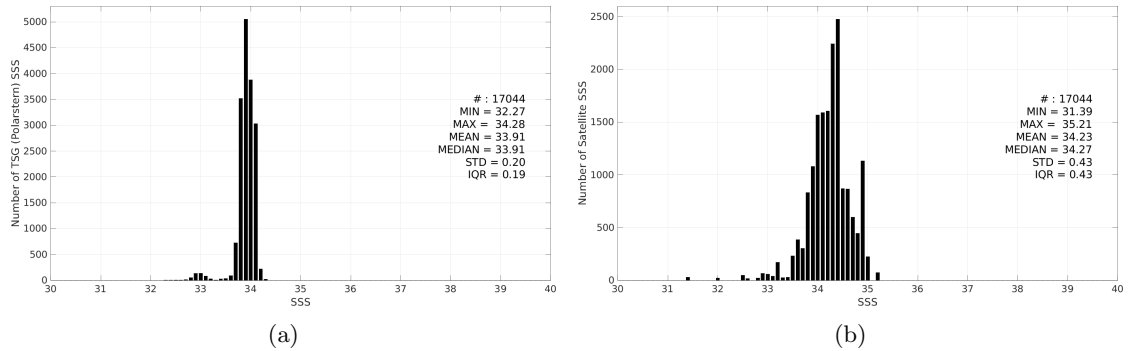
Figure 3: Histograms of SSS from TSG (Polarstern) (a) and Aquarius SSS L3 CAP v5 - Monthly (JPL) (b) considering all match-up pairs per bins of 0.1 over the Southern Ocean Pi-MEP region and for the full satellite product period.
