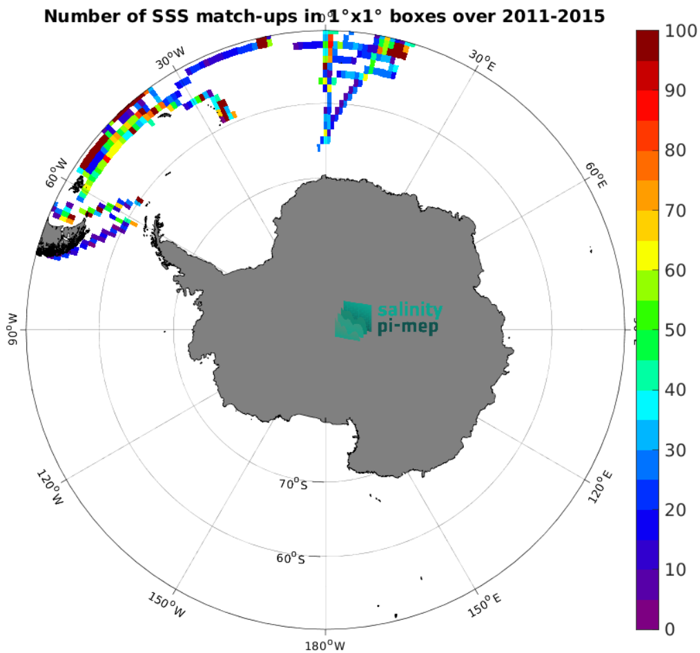
Figure 5: Number of SSS match-ups between TSG (Polarstern) SSS and the Aquarius SSS L3 CAP v5 - Monthly (JPL) SSS product for the Southern Ocean Pi-MEP region over 1^\circ \times 1^\circ boxes and for the full satellite product period.
