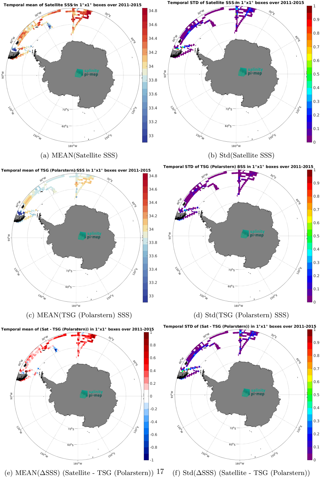
Figure 7: Temporal mean (left) and Std (right) of SSS from Aquarius SSS L3 CAP v5 - Monthly (JPL) (top), TSG (Polarstern) (middle), and of \Delta SSS (Satellite - TSG (Polarstern)). Only match-up pairs are used to generate these maps.
