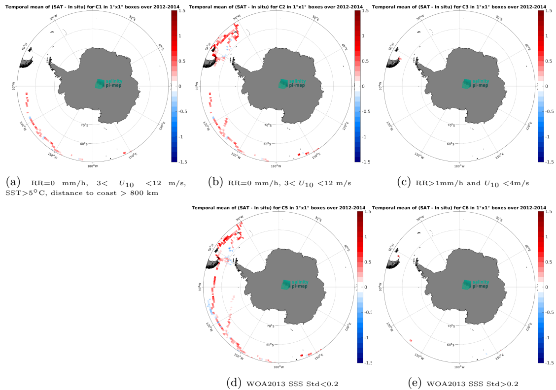
Figure 12: Temporal mean gridded over spatial boxes of size 1^\circ \times 1^\circ of \Delta\text{SSS} (Aquarius SSS L3 CAP v5 - Monthly (JPL) - TSG (GOSUD-Sailing-ship)) for 5 different subdatasets corresponding to: RR=0 mm/h, 3 < U_{10} < 12 m/s, SST > 5^\circ\text{C} , distance to coast > 800 km (a), RR=0 mm/h, 3 < U_{10} < 12 m/s (b), RR > 1 mm/h and U_{10} < 4 m/s (c), WOA2013 SSS Std < 0.2 (d), WOA2013 SSS Std > 0.2 (e).
