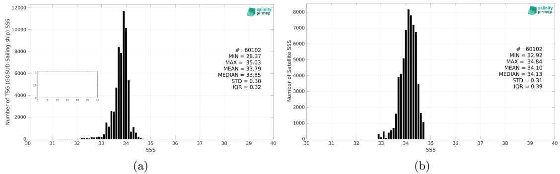
Figure 2: Histograms of SSS from TSG (GOSUD-Sailing-ship) (a) and Aquarius SSS L3 CAP v5 - Monthly (JPL) (b) considering all match-up pairs per bins of 0.1 over the Southern Ocean Pi-MEP region and for the full satellite product period.
