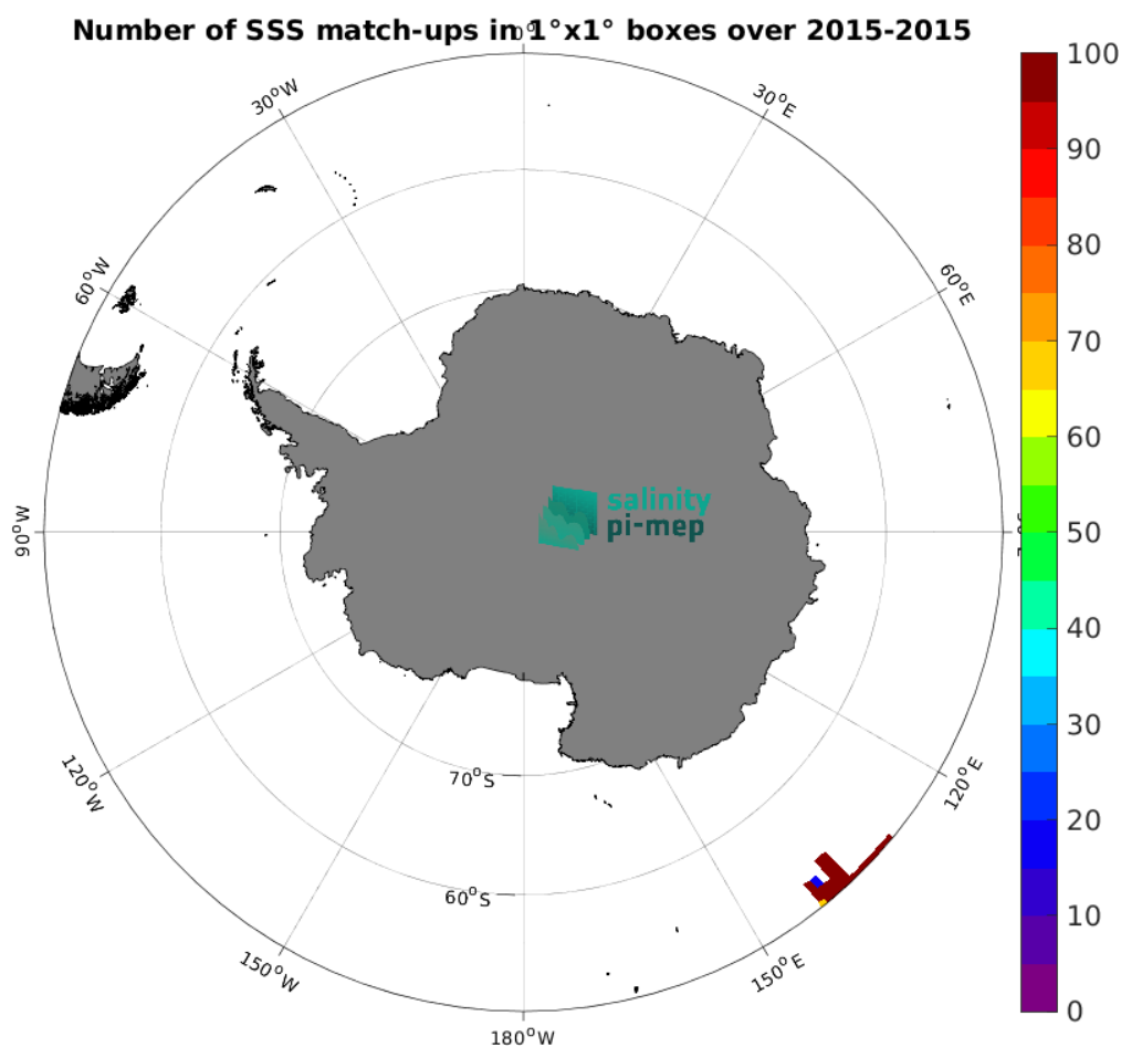
Figure 4: Number of SSS match-ups between TSG (GOSUD-Research-vessel) SSS and the Aquarius SSS L3 CAP v5 - Monthly (JPL) SSS product for the Southern Ocean Pi-MEP region over 1^\circ \times 1^\circ boxes and for the full satellite product period.
