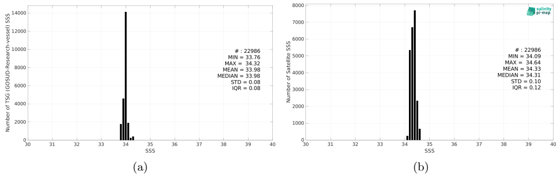
Figure 2: Histograms of SSS from TSG (GOSUD-Research-vessel) (a) and Aquarius SSS L3 CAP v5 - Monthly (JPL) (b) considering all match-up pairs per bins of 0.1 over the Southern Ocean Pi-MEP region and for the full satellite product period.
