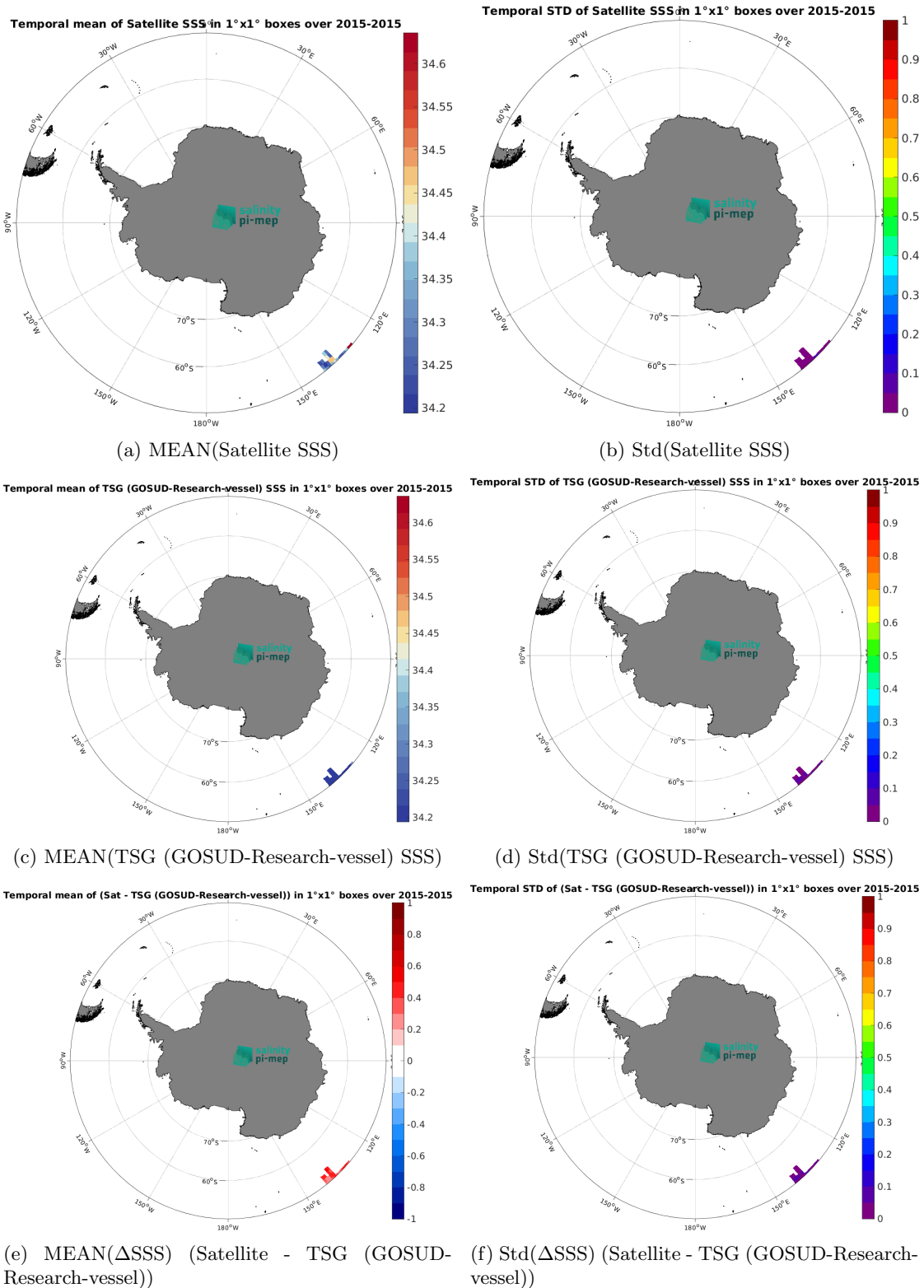
Figure 6: Temporal mean (left) and Std (right) of SSS from Aquarius SSS L3 CAP v5 - Monthly (JPL) (top), TSG (GOSUD-Research-vessel) (middle), and of \Delta SSS (Satellite - TSG (GOSUD-Research-vessel)). Only match-up pairs are used to generate these maps.
