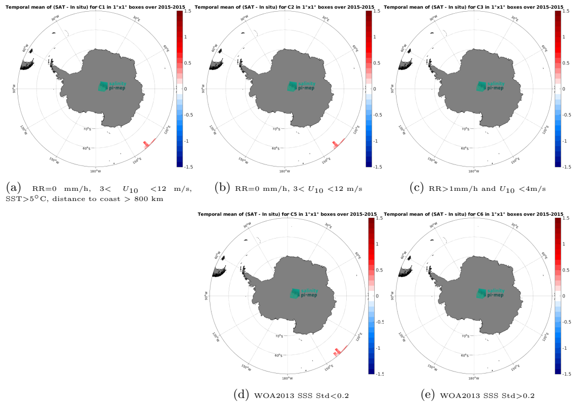
Figure 12: Temporal mean gridded over spatial boxes of size 1^\circ \times 1^\circ of \Delta\text{SSS} (Aquarius SSS L3 CAP v5 - Monthly (JPL) - TSG (GOSUD-Research-vessel)) for 5 different subdatasets corresponding to: RR=0 mm/h, 3 < U_{10} < 12 m/s, SST > 5^\circ\text{C} , distance to coast > 800 km (a), RR=0 mm/h, 3 < U_{10} < 12 m/s (b), RR > 1 mm/h and U_{10} < 4 m/s (c), WOA2013 SSS Std < 0.2 (d), WOA2013 SSS Std > 0.2 (e).
