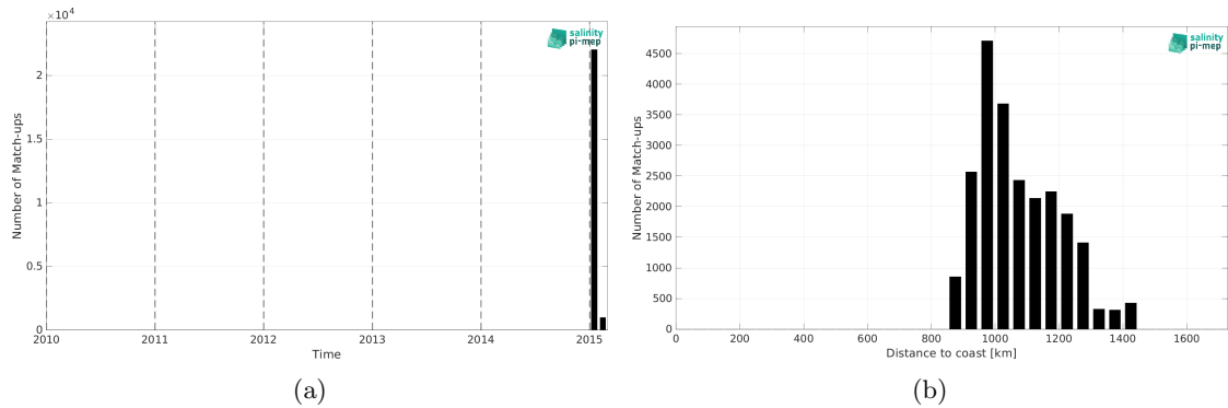
Figure 1: Number of match-ups between TSG (GOSUD-Research-vessel) and Aquarius SSS L3 CAP v5 - Monthly (JPL) SSS as a function of time (a) and as function of the distance to coast (b) over the Southern Ocean Pi-MEP region and for the full satellite product period.
