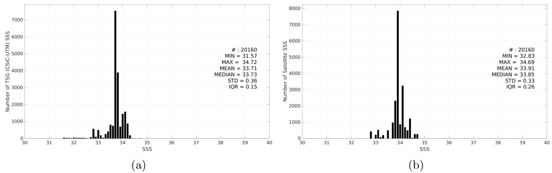
Figure 3: Histograms of SSS from TSG (CSIC-UTM) (a) and Aquarius SSS L3 CAP v5 - Monthly (JPL) (b) considering all match-up pairs per bins of 0.1 over the Southern Ocean Pi-MEP region and for the full satellite product period.
