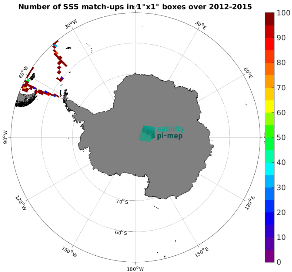
Figure 5: Number of SSS match-ups between TSG (CSIC-UTM) SSS and the Aquarius SSS L3 CAP v5 - Monthly (JPL) SSS product for the Southern Ocean Pi-MEP region over 1^{\circ} \times 1^{\circ} boxes and for the full satellite product period.
