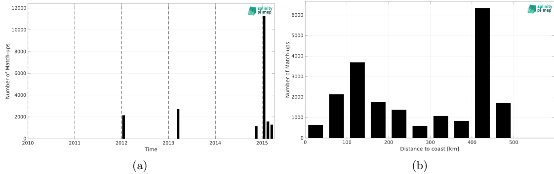
Figure 2: Number of match-ups between TSG (CSIC-UTM) and Aquarius SSS L3 CAP v5 - Monthly (JPL) SSS as a function of time (a) and as function of the distance to coast (b) over the Southern Ocean Pi-MEP region and for the full satellite product period.
