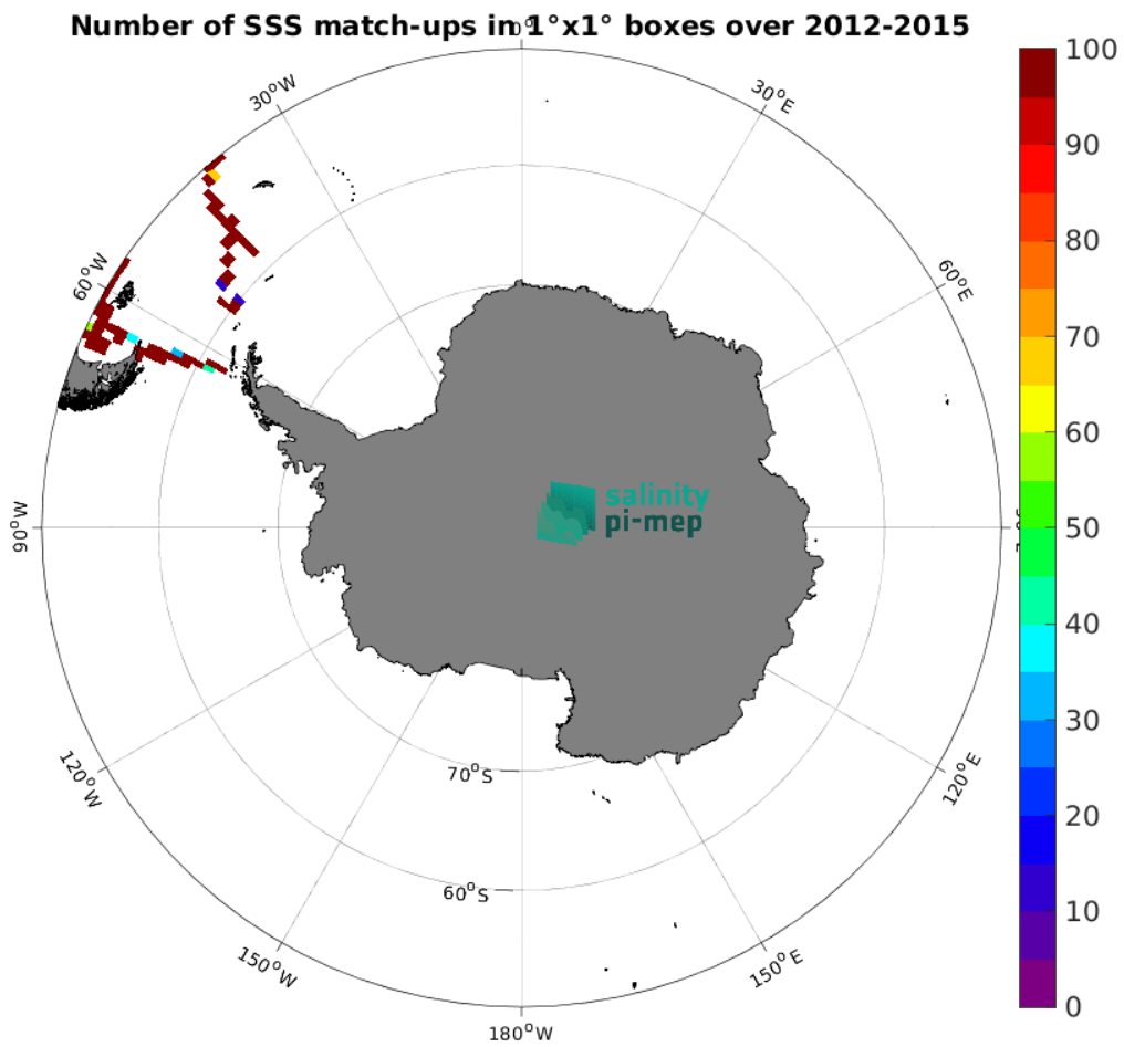
Figure 4: Number of SSS match-ups between TSG (CSIC-UTM) SSS and the Aquarius SSS L3 CAP v5 - Monthly (JPL) SSS product for the Southern Ocean Pi-MEP region over 1^{\circ} \times 1^{\circ} boxes and for the full satellite product period.
