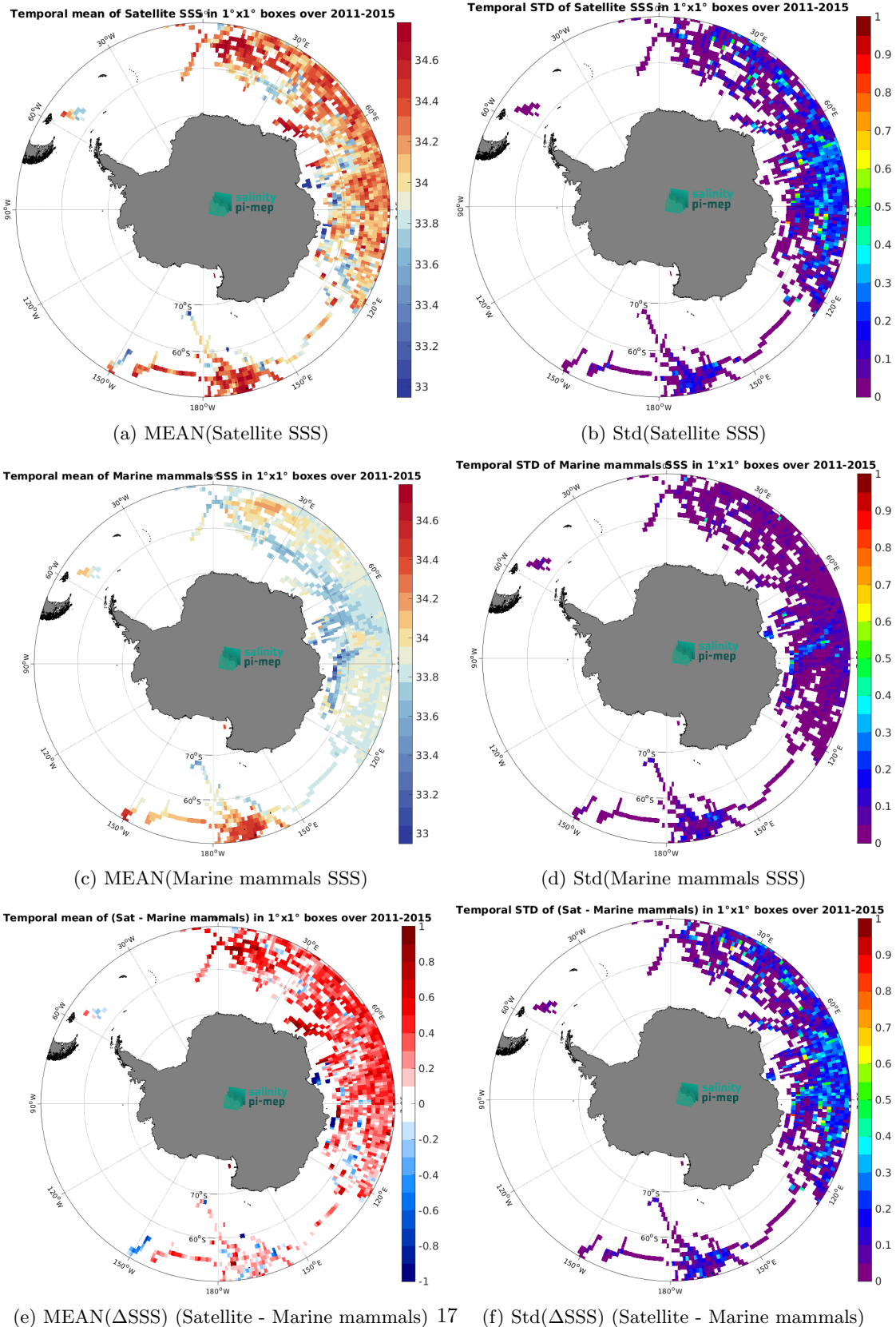
Figure 7: Temporal mean (left) and Std (right) of SSS from Aquarius SSS L3 CAP v5 - Monthly (JPL) (top), Marine mammals (middle), and of \Delta SSS (Satellite - Marine mammals). Only match-up pairs are used to generate these maps.
