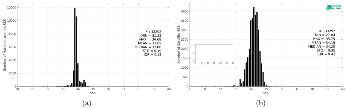
Figure 3: Histograms of SSS from Marine mammals (a) and Aquarius SSS L3 CAP v5 - Monthly (JPL) (b) considering all match-up pairs per bins of 0.1 over the Southern Ocean Pi-MEP region and for the full satellite product period.
