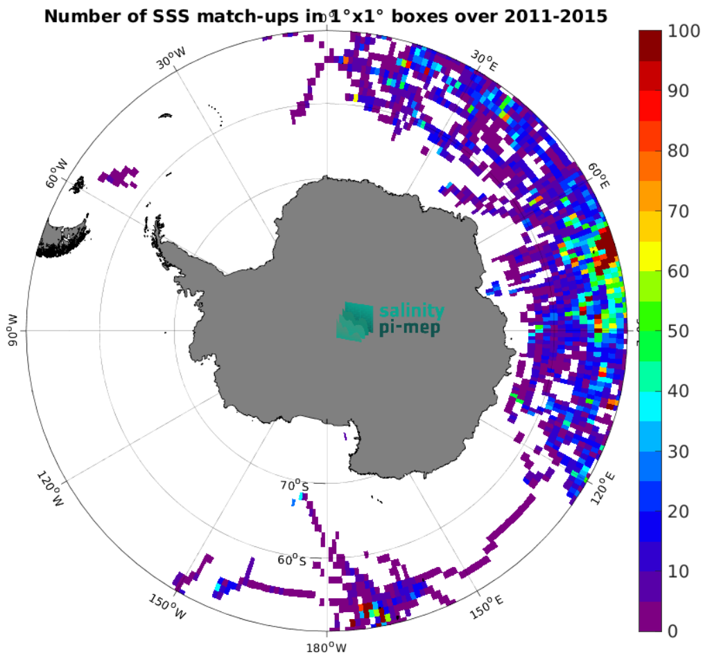
Figure 5: Number of SSS match-ups between Marine mammals SSS and the Aquarius SSS L3 CAP v5 - Monthly (JPL) SSS product for the Southern Ocean Pi-MEP region over 1^\circ \times 1^\circ boxes and for the full satellite product period.
