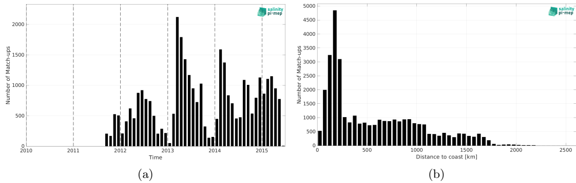
Figure 2: Number of match-ups between Marine mammals and Aquarius SSS L3 CAP v5 - Monthly (JPL) SSS as a function of time (a) and as function of the distance to coast (b) over the Southern Ocean Pi-MEP region and for the full satellite product period.
