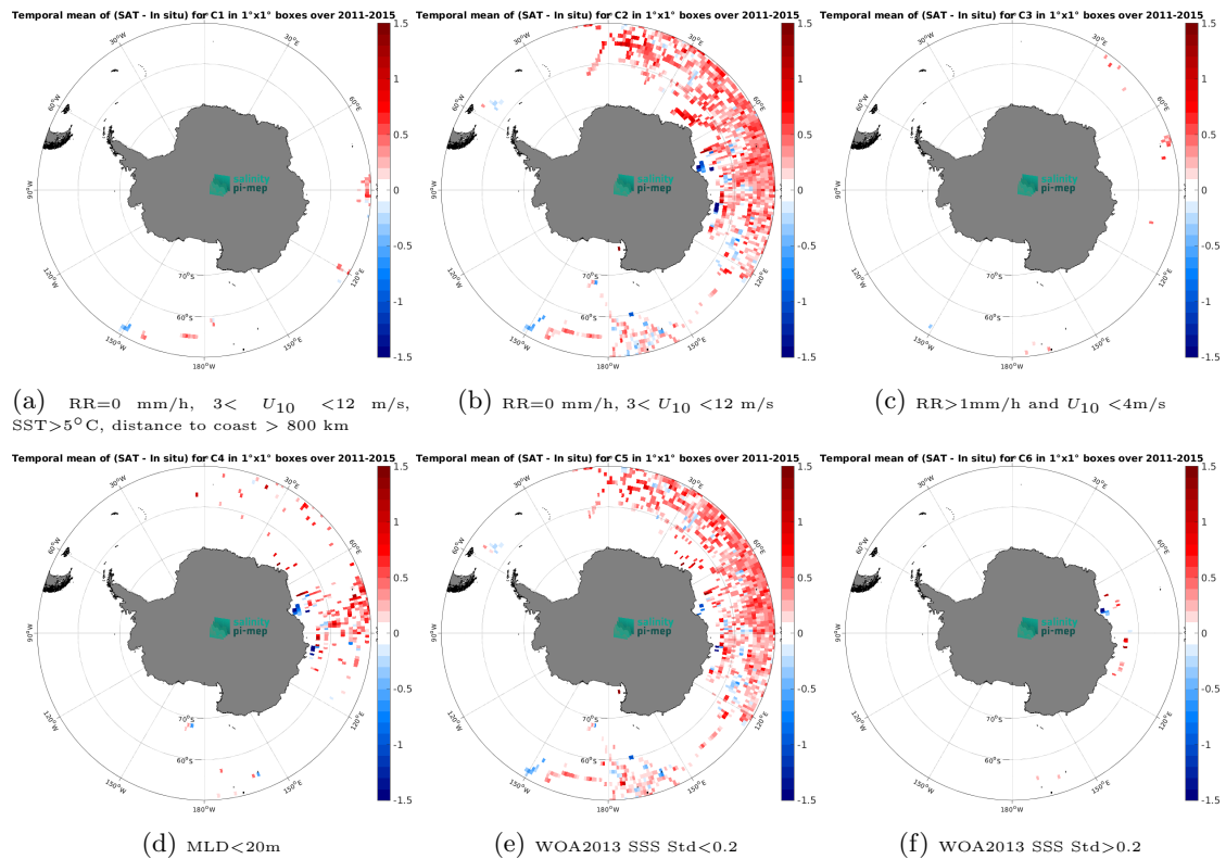
Figure 14: Temporal mean gridded over spatial boxes of size 1^\circ \times 1^\circ of \Delta SSS (Aquarius SSS L3 CAP v5 - Monthly (JPL) - Marine mammals) for 6 different subdatasets corresponding to:RR=0 mm/h, 3 < U_{10} < 12 m/s, SST>5°C, distance to coast > 800 km (a), RR=0 mm/h, 3 < U_{10} < 12 m/s (b), RR>1mm/h and U_{10} < 4 m/s (c),MLD<20m (d),WOA2013 SSS Std<0.2 (e),WOA2013 SSS Std>0.2 (f).
