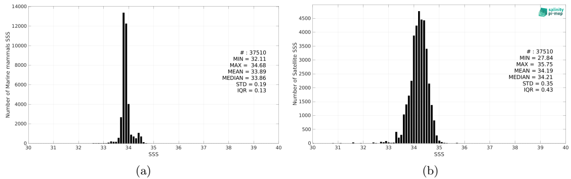
Figure 2: Histograms of SSS from Marine mammals (a) and Aquarius SSS L3 CAP v5 - Monthly (JPL) (b) considering all match-up pairs per bins of 0.1 over the Southern Ocean Pi-MEP region and for the full satellite product period.
