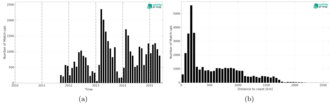
Figure 1: Number of match-ups between Marine mammals and Aquarius SSS L3 CAP v5 - Monthly (JPL) SSS as a function of time (a) and as function of the distance to coast (b) over the Southern Ocean Pi-MEP region and for the full satellite product period.
