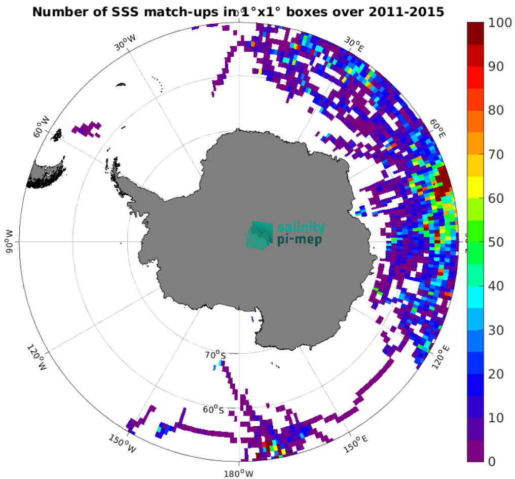
Figure 4: Number of SSS match-ups between Marine mammals SSS and the Aquarius SSS L3 CAP v5 - Monthly (JPL) SSS product for the Southern Ocean Pi-MEP region over 1^\circ \times 1^\circ boxes and for the full satellite product period.
