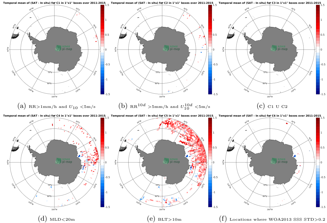
Figure 12: Temporal mean gridded over spatial boxes of size 1^\circ \times 1^\circ of \Delta\text{SSS} (Aquarius-L3-JPL-V5-MONTHLY - Sea mammals) for 6 different subdatasets corresponding to:RR >1\text{mm/h} and U_{10} < 5\text{m/s} (a), RR^{10d} > 5\text{mm/h} and U_{10}^{10d} < 5\text{m/s} (b), C1 U C2 (c),MLD <20\text{m} (d),BLT >10\text{m} (e),Locations where WOA2013 SSS STD >0.2 (f).
