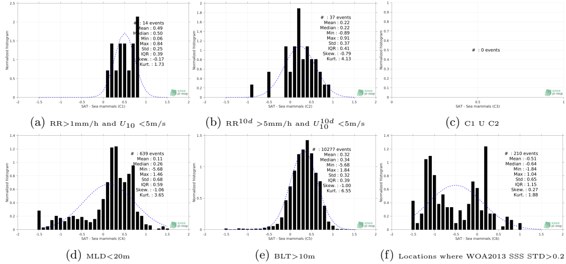
Figure 13: Normalized histogram of \Delta SSS (Aquarius-L3-JPL-V5-MONTHLY - Sea mammals) for 6 different subdatasets corresponding to: RR > 1mm/h and U_{10} < 5m/s (a), RR^{10d} > 5mm/h and U_{10}^{10d} < 5m/s (b), C1 U C2 (c), MLD < 20m (d), BLT > 10m (e), Locations where WOA2013 SSS STD > 0.2 (f).
