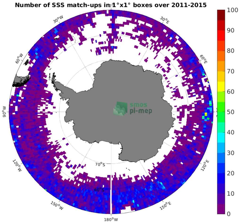
Figure 4: Number of SSS match-ups between Argo SSS and the Aquarius SSS L3 CAP v5 - Monthly (JPL) SSS product for the Southern Ocean Pi-MEP region over 1^\circ \times 1^\circ boxes and for the full satellite product period.
