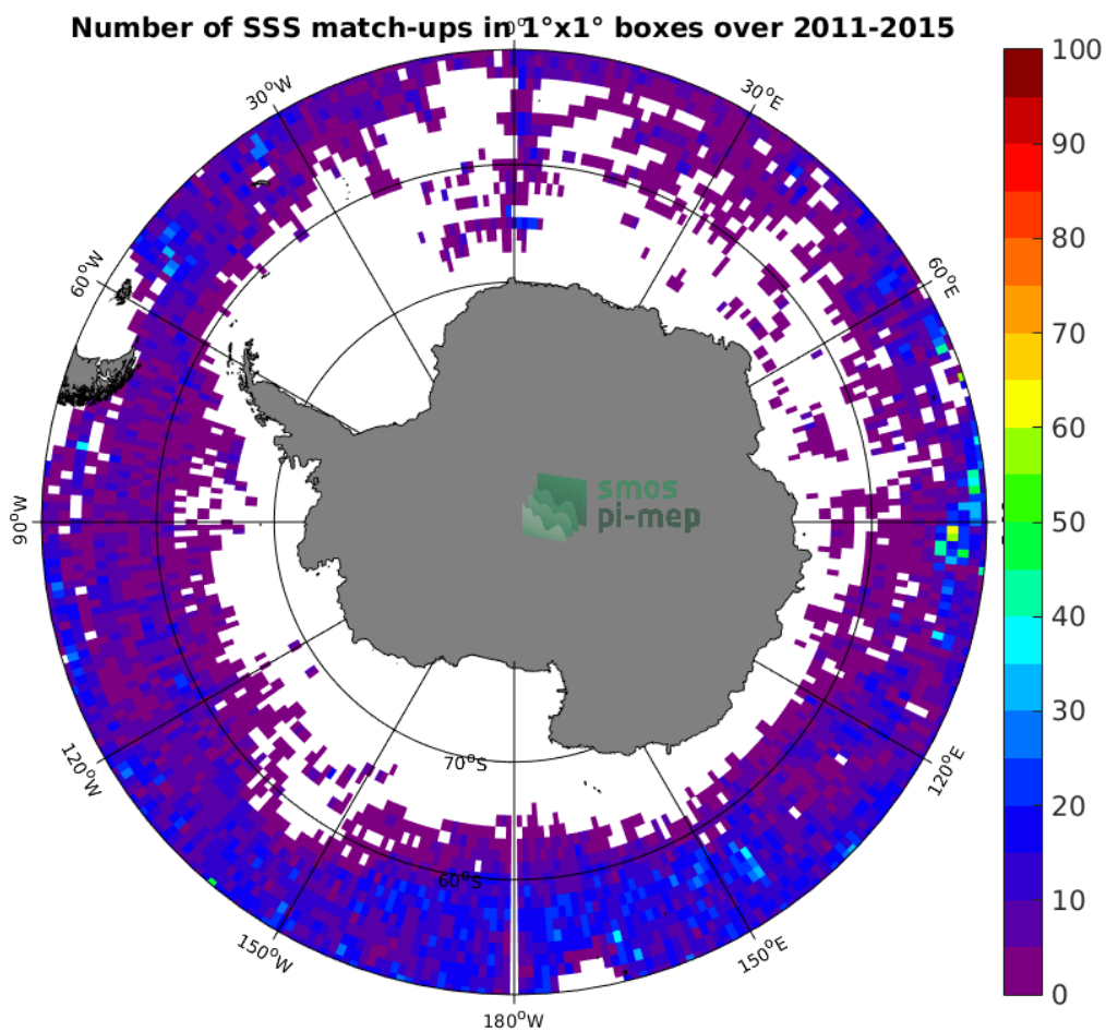
Figure 4: Number of SSS match-ups between Argo SSS and the Aquarius-L3-JPL-V5-MONTHLY SSS product for the Southern Ocean Pi-MEP region over 1°x1° boxes and for the full satellite product period.
