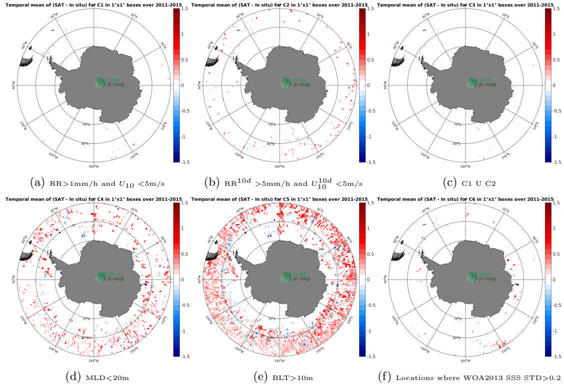
Figure 12: Temporal mean gridded over spatial boxes of size 1^\circ \times 1^\circ of \Delta SSS (Aquarius-L3-JPL-V5-MONTHLY - Argo) for 6 different subdatasets corresponding to: RR > 1\text{mm/h} and U_{10} < 5\text{m/s} (a), RR^{10d} > 5\text{mm/h} and U_{10}^{10d} < 5\text{m/s} (b), C1 U C2 (c), MLD < 20\text{m} (d), BLT > 10\text{m} (e), Locations where WOA2013 SSS STD > 0.2 (f).
