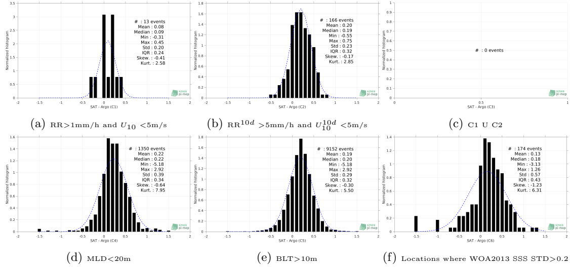
Figure 13: Normalized histogram of \Delta SSS (Aquarius-L3-JPL-V5-MONTHLY - Argo) for 6 different subdatasets corresponding to: RR > 1mm/h and U_{10} < 5 m/s (a), RR^{10d} > 5 mm/h and U_{10}^{10d} < 5 m/s (b), C1 U C2 (c), MLD < 20m (d), BLT > 10m (e), Locations where WOA2013 SSS STD > 0.2 (f).
