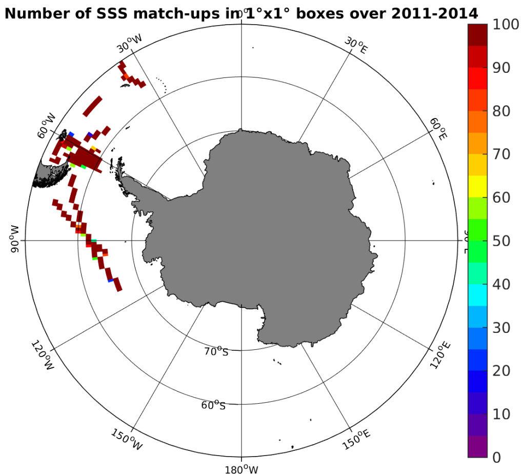
Figure 4: Number of SSS match-ups between TSG-SAMOS SSS and the Aquarius-L3-JPL-V4-MONTHLY SSS product for the Southern Ocean Pi-MEP region over 1°x1° boxes and for the full satellite product period.
