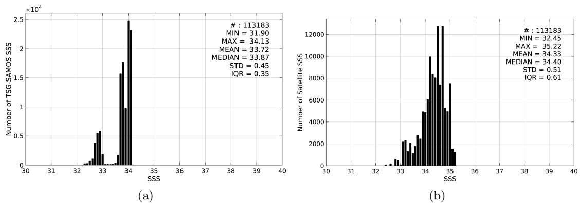
Figure 2: Histograms of SSS from TSG-SAMOS (a) and Aquarius-L3-JPL-V4-MONTHLY (b) considering all match-up pairs per bins of 0.1 over the Southern Ocean Pi-MEP region and for the full satellite product period.
