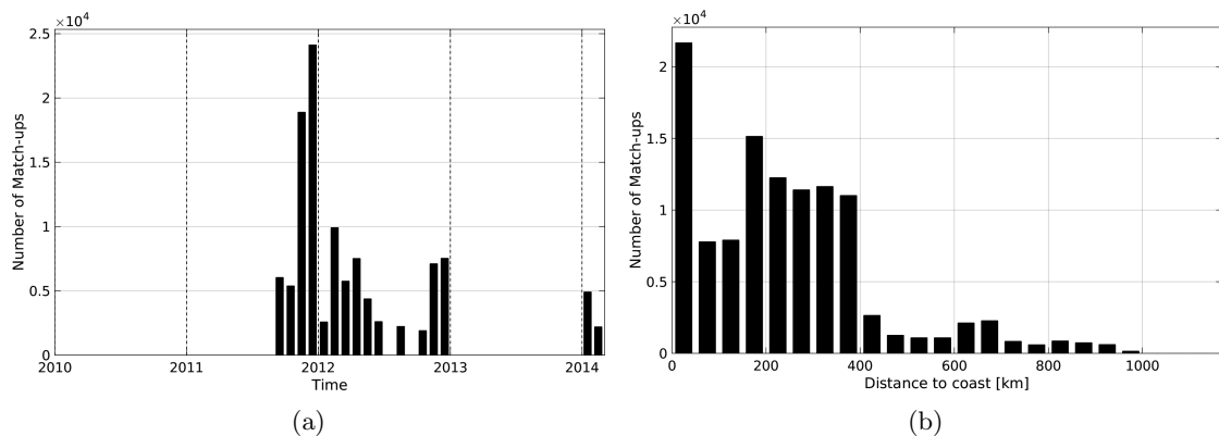
Figure 1: Number of match-ups between TSG-SAMOS and Aquarius-L3-JPL-V4-MONTHLY SSS as a function of time (a) and as function of the distance to coast (b) over the Southern Ocean Pi-MEP region and for the full satellite product period.
