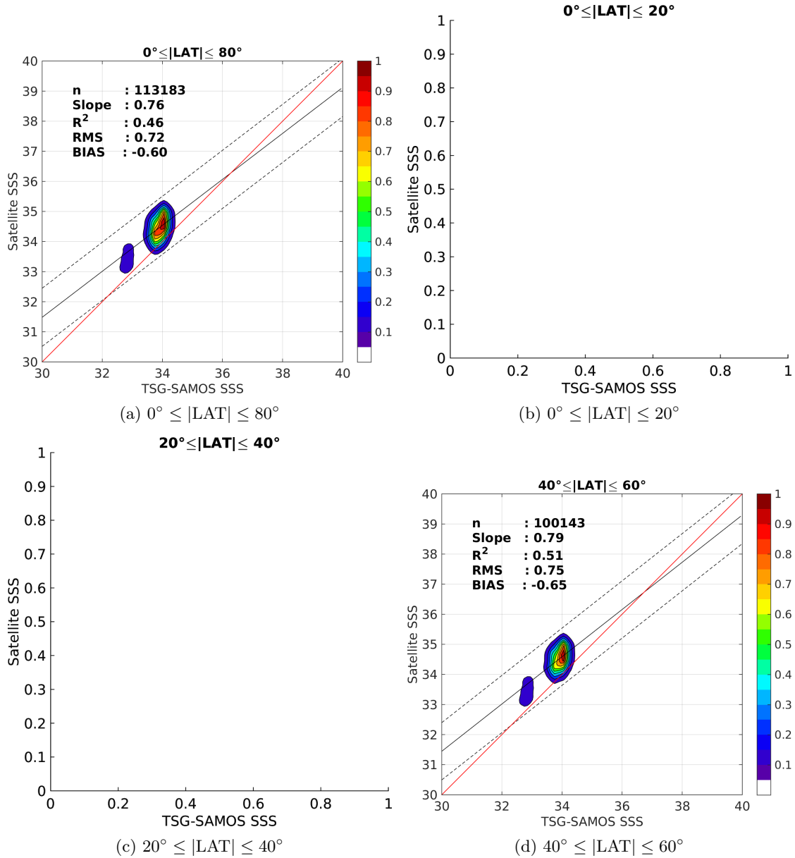
Figure 9: Contour maps of the concentration of Aquarius-L3-JPL-V4-MONTHLY SSS (y-axis) versus TSG-SAMOS SSS (x-axis) at match-up pairs for different latitude bands. For each plot, the red line shows x=y . The black thin and dashed lines indicate a linear fit through the data cloud and the \pm 95\% confidence levels, respectively. The number match-up pairs n , the slope and R^2 coefficient of the linear fit, the root mean square (RMS) and the mean bias between satellite and in situ data are indicated for each latitude band in each plots.
