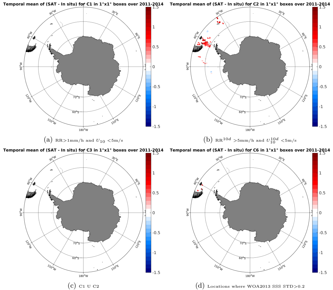
Figure 12: Temporal mean gridded over spatial boxes of size 1°x1° of \Delta SSS (Aquarius-L3-JPL-V4-MONTHLY - TSG-SAMOS) for 4 different subdatasets corresponding to: RR > 1\text{mm/h} and U_{10} < 5\text{m/s} (a), RR^{10d} > 5\text{mm/h} and U_{10}^{10d} < 5\text{m/s} (b), C1 U C2 (c), Locations where WOA2013 SSS STD > 0.2 (d).
