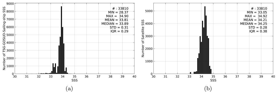
Figure 2: Histograms of SSS from TSG-GOSUD-Sailing-ship (a) and Aquarius-L3-JPL-V4-MONTHLY (b) considering all match-up pairs per bins of 0.1 over the Southern Ocean Pi-MEP region and for the full satellite product period.
