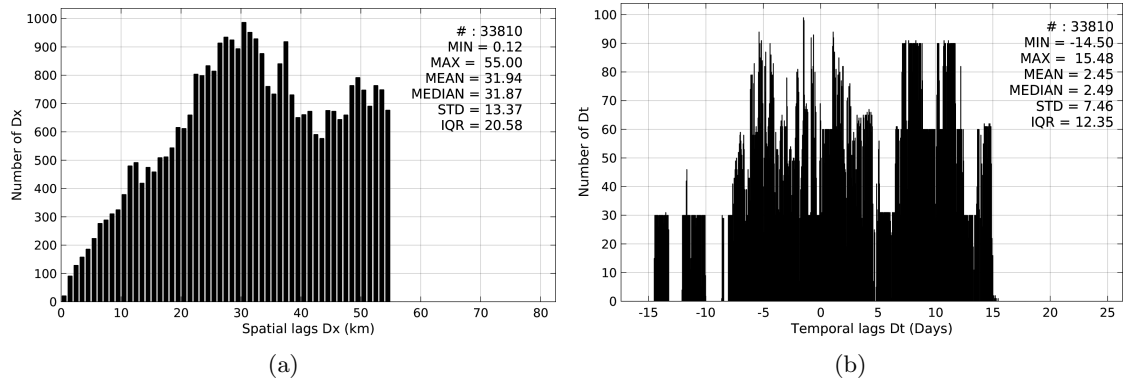
Figure 5: Histograms of the spatial (a) and temporal (b) lags between the time of the TSG-GOSUD-Sailing-ship measurements and the date of the corresponding Aquarius-L3-JPL-V4-MONTHLY SSS product.
