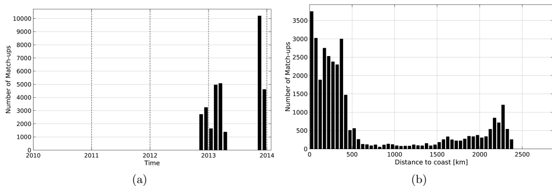
Figure 1: Number of match-ups between TSG-GOSUD-Sailing-ship and Aquarius-L3-JPL-V4-MONTHLY SSS as a function of time (a) and as function of the distance to coast (b) over the Southern Ocean Pi-MEP region and for the full satellite product period.
