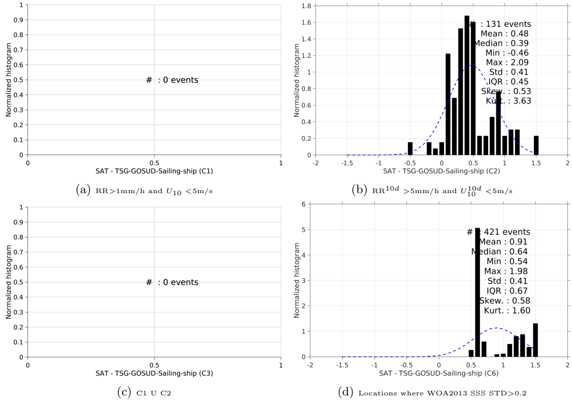
Figure 13: Normalized histogram of \Delta\text{SSS} (Aquarius-L3-JPL-V4-MONTHLY - TSG-GOSUD-Sailing-ship) for 6 different subdatasets corresponding to: RR > 1\text{mm/h} and U_{10} < 5\text{m/s} (a), RR^{10d} > 5\text{mm/h} and U_{10}^{10d} < 5\text{m/s} (b), C1 U C2 (c), Locations where WOA2013 SSS STD > 0.2 (d).
