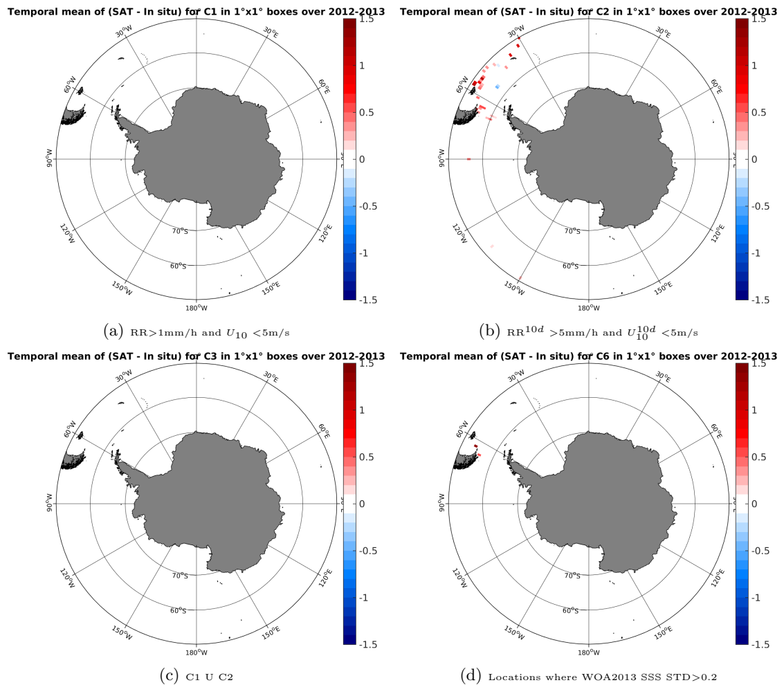
Figure 12: Temporal mean gridded over spatial boxes of size 1^\circ \times 1^\circ of \Delta SSS (Aquarius-L3-JPL-V4-MONTHLY - TSG-GOSUD-Sailing-ship) for 4 different subdatasets corresponding to: RR > 1\text{mm/h} and U_{10} < 5\text{m/s} (a), RR^{10d} > 5\text{mm/h} and U_{10}^{10d} < 5\text{m/s} (b), C1 U C2 (c), Locations where WOA2013 SSS STD > 0.2 (d).
