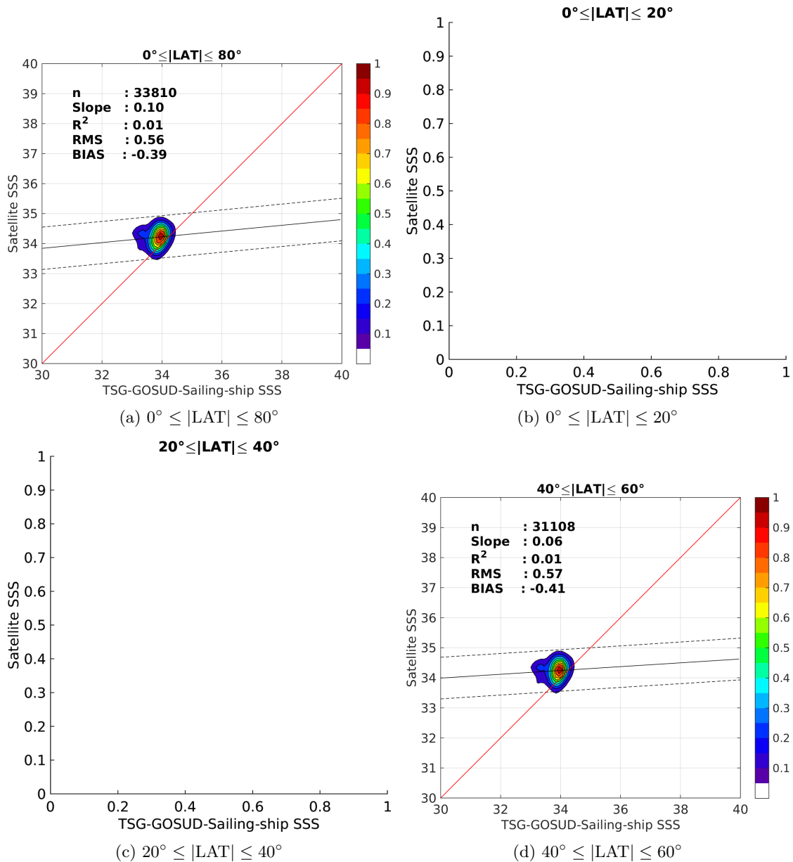
Figure 9: Contour maps of the concentration of Aquarius-L3-JPL-V4-MONTHLY SSS (y-axis) versus TSG-GOSUD-Sailing-ship SSS (x-axis) at match-up pairs for different latitude bands. For each plot, the red line shows x=y . The black thin and dashed lines indicate a linear fit through the data cloud and the \pm 95\% confidence levels, respectively. The number match-up pairs n , the slope and R^2 coefficient of the linear fit, the root mean square (RMS) and the mean bias between satellite and in situ data are indicated for each latitude band in each plots.
