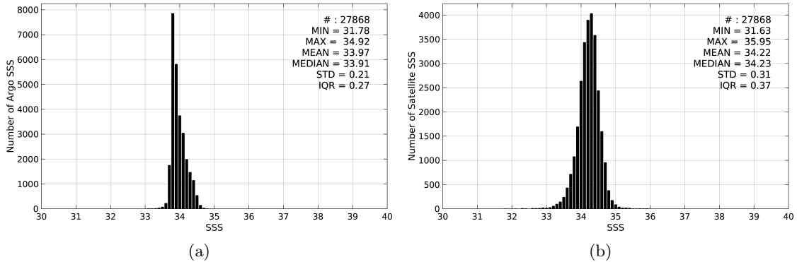
Figure 2: Histograms of SSS from Argo (a) and Aquarius-L3-JPL-V4-MONTHLY (b) considering all match-up pairs per bins of 0.1 over the Southern Ocean Pi-MEP region and for the full satellite product period.
