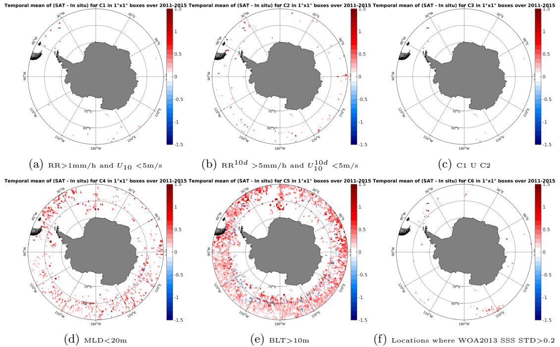
Figure 12: Temporal mean gridded over spatial boxes of size 1^\circ \times 1^\circ of \Delta SSS (Aquarius-L3-JPL-V4-MONTHLY - Argo) for 6 different subdatasets corresponding to: RR > 1\text{mm/h} and U_{10} < 5\text{m/s} (a), RR^{10d} > 5\text{mm/h} and U_{10}^{10d} < 5\text{m/s} (b), C1 U C2 (c), MLD < 20\text{m} (d), BLT > 10\text{m} (e), Locations where WOA2013 SSS STD > 0.2 (f).
