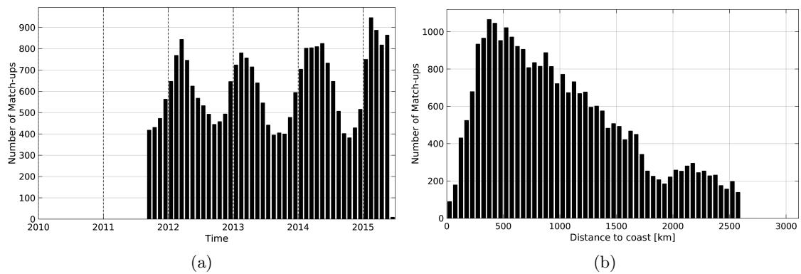
Figure 1: Number of match-ups between Argo and Aquarius-L3-JPL-V4-MONTHLY SSS as a function of time (a) and as function of the distance to coast (b) over the Southern Ocean Pi-MEP region and for the full satellite product period.
