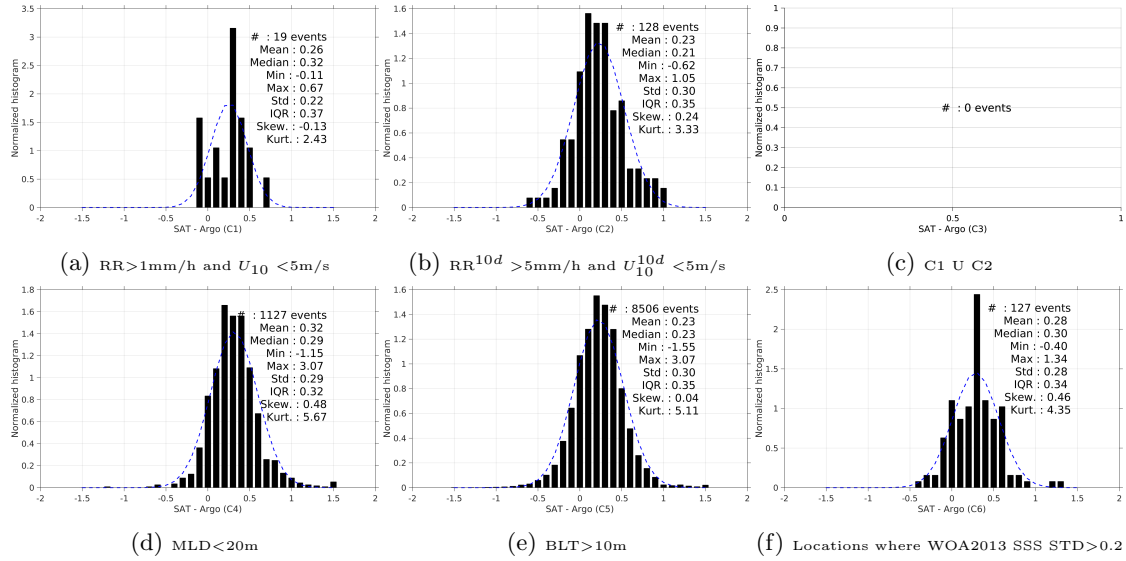
Figure 13: Normalized histogram of \Delta SSS (Aquarius-L3-JPL-V4-MONTHLY - Argo) for 6 different subdatasets corresponding to: RR>1mm/h and U_{10} < 5\text{m/s} (a), RR 10d >5mm/h and U_{10}^{10d} < 5\text{m/s} (b), C1 U C2 (c),MLD<20m (d),BLT>10m (e),Locations where WOA2013 SSS STD>0.2 (f).
