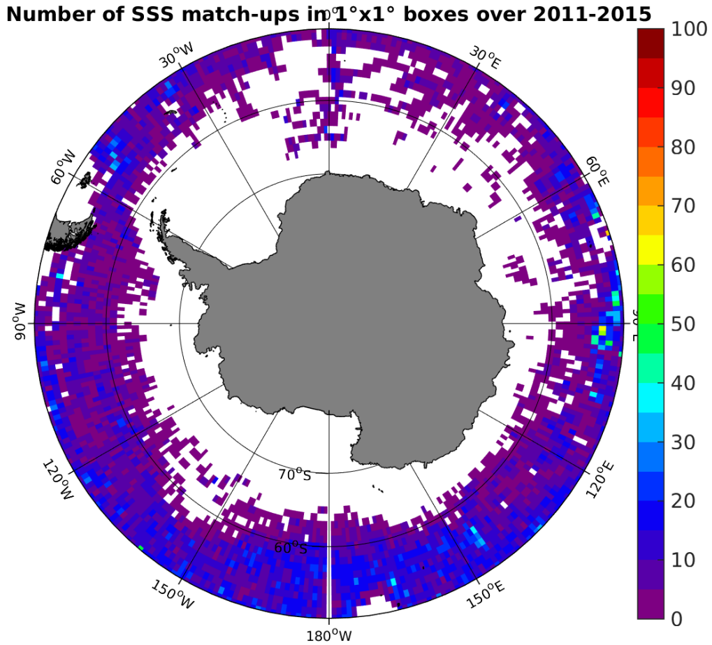
Figure 4: Number of SSS match-ups between Argo SSS and the Aquarius-L3-JPL-V4-MONTHLY SSS product for the Southern Ocean Pi-MEP region over 1^\circ \times 1^\circ boxes and for the full satellite product period.
