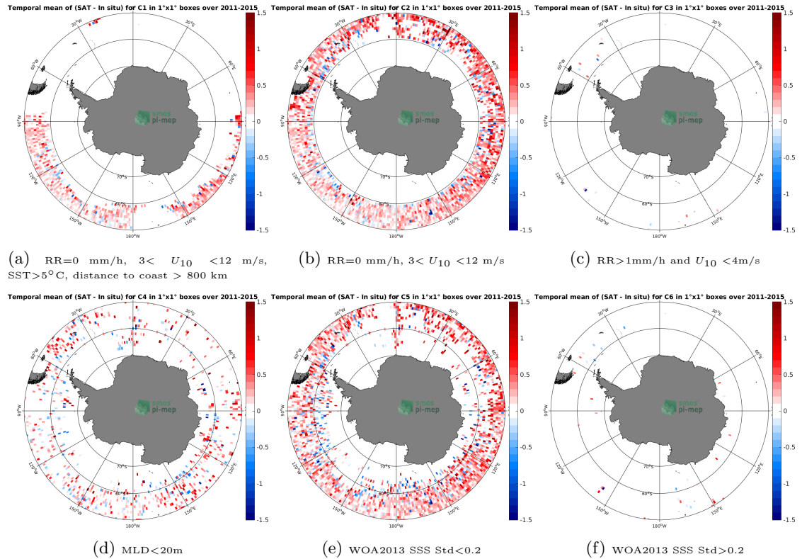
Figure 12: Temporal mean gridded over spatial boxes of size 1^{\circ}\times 1^{\circ} of \Delta\text{SSS} (Aquarius SSS L2-AVERAGED CAP v5 (JPL) - Argo) for 6 different subdatasets corresponding to:RR=0 mm/h, 3 < U_{10} < 12 m/s, SST >5^{\circ}\text{C} , distance to coast > 800 km (a), RR=0 mm/h, 3 < U_{10} < 12 m/s (b), RR >1 mm/h and U_{10} < 4 m/s (c),MLD <20 m (d),WOA2013 SSS Std <0.2 (e),WOA2013 SSS Std >0.2 (f).
