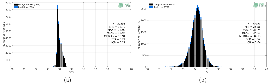
Figure 2: Histograms of SSS from Argo (a) and Aquarius SSS L2-AVERAGED CAP v5 (JPL) (b) considering all match-up pairs per bins of 0.1 over the Southern Ocean Pi-MEP region and for the full satellite product period.
