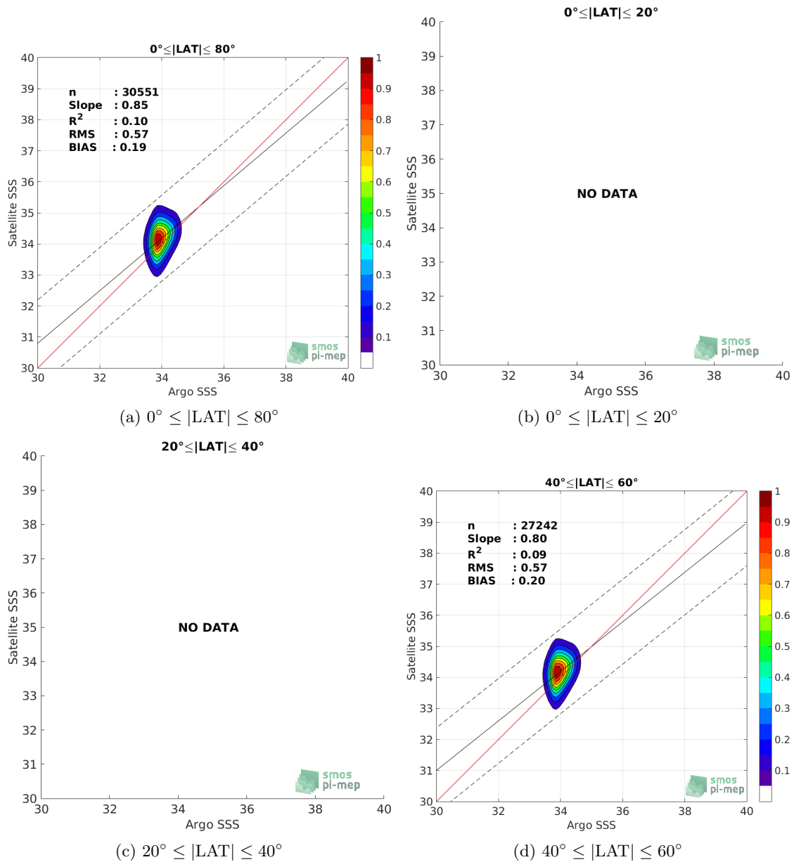
Figure 9: Contour maps of the concentration of Aquarius SSS L2-AVERAGED CAP v5 (JPL) SSS (y-axis) versus Argo SSS (x-axis) at match-up pairs for different latitude bands. For each plot, the red line shows x=y . The black thin and dashed lines indicate a linear fit through the data cloud and the \pm 95\% confidence levels, respectively. The number match-up pairs n , the slope and R^2 coefficient of the linear fit, the root mean square (RMS) and the mean bias between satellite and in situ data are indicated for each latitude band in each plot.
