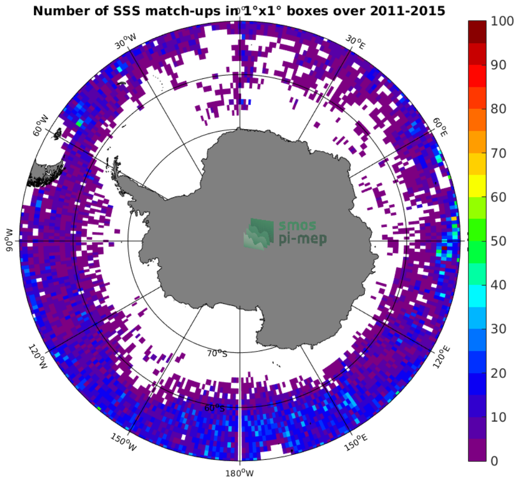
Figure 4: Number of SSS match-ups between Argo SSS and the Aquarius SSS L2-AVERAGED CAP v5 (JPL) SSS product for the Southern Ocean Pi-MEP region over 1^\circ \times 1^\circ boxes and for the full satellite product period.
