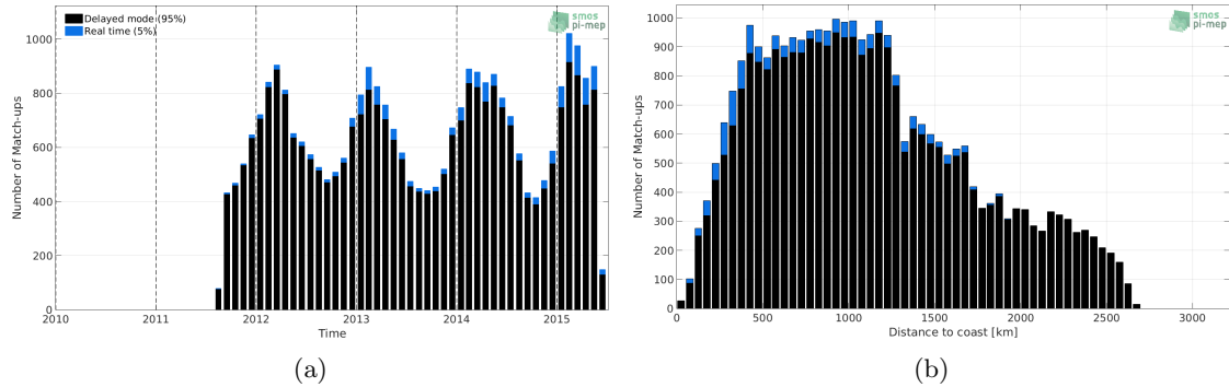
Figure 1: Number of match-ups between Argo and Aquarius SSS L2-AVERAGED CAP v5 (JPL) SSS as a function of time (a) and as function of the distance to coast (b) over the Southern Ocean Pi-MEP region and for the full satellite product period.
