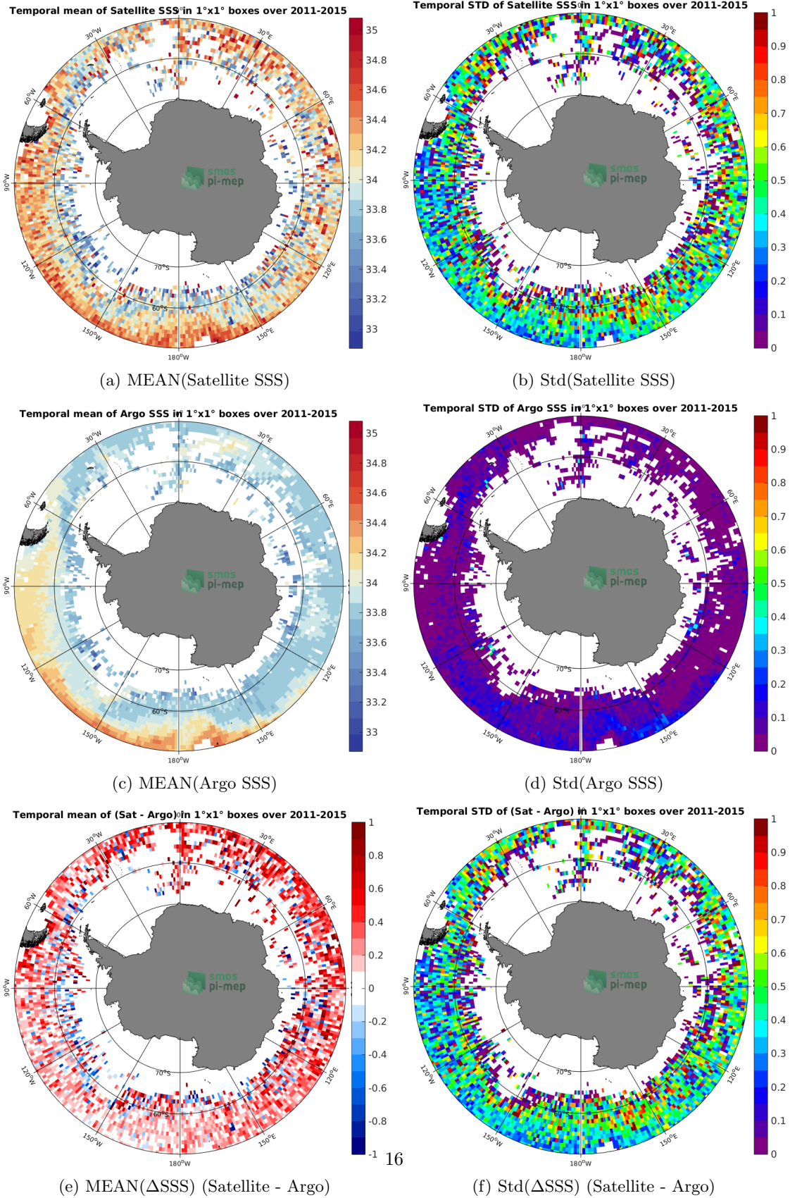
Figure 6: Temporal mean (left) and Std (right) of SSS from Aquarius SSS L2-AVERAGED CAP v5 (JPL) (top), Argo (middle), and of \Delta SSS (Satellite - Argo). Only match-up pairs are used to generate these maps.
