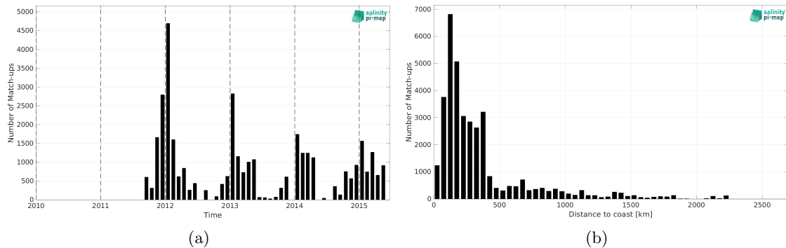
Figure 2: Number of match-ups between TSG (SAMOS) and Aquarius SSS L2 OR v5 (NASA-GSFC) SSS as a function of time (a) and as function of the distance to coast (b) over the Southern Ocean Pi-MEP region and for the full satellite product period.
