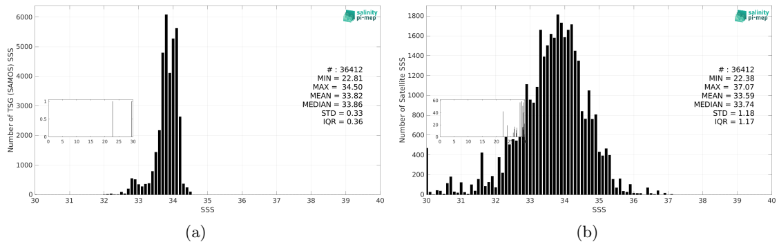
Figure 3: Histograms of SSS from TSG (SAMOS) (a) and Aquarius SSS L2 OR v5 (NASA-GSFC) (b) considering all match-up pairs per bins of 0.1 over the Southern Ocean Pi-MEP region and for the full satellite product period.
