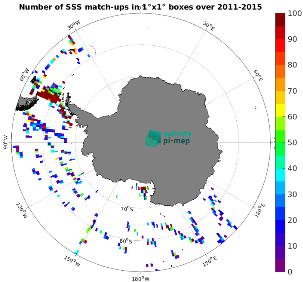
Figure 5: Number of SSS match-ups between TSG (SAMOS) SSS and the Aquarius SSS L2 OR v5 (NASA-GSFC) SSS product for the Southern Ocean Pi-MEP region over 1^\circ \times 1^\circ boxes and for the full satellite product period.
