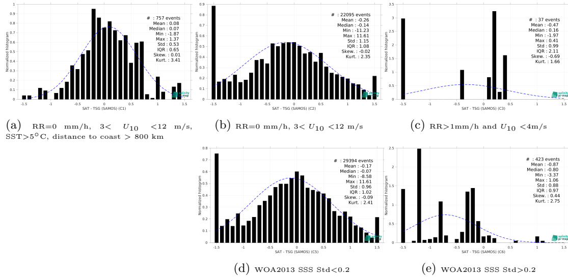
Figure 15: Normalized histogram of \Delta SSS (Aquarius SSS L2 OR v5 (NASA-GSFC) - TSG (SAMOS)) for 5 different subdatasets corresponding to: RR=0 mm/h, 3 < U_{10} < 12 m/s, SST > 5°C, distance to coast > 800 km (a), RR=0 mm/h, 3 < U_{10} < 12 m/s (b), RR > 1mm/h and U_{10} < 4 m/s (c), WOA2013 SSS Std < 0.2 (d), WOA2013 SSS Std > 0.2 (e).
