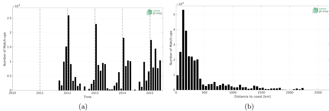
Figure 1: Number of match-ups between TSG (SAMOS) and Aquarius SSS L2 OR v5 (NASA-GSFC) SSS as a function of time (a) and as function of the distance to coast (b) over the Southern Ocean Pi-MEP region and for the full satellite product period.
