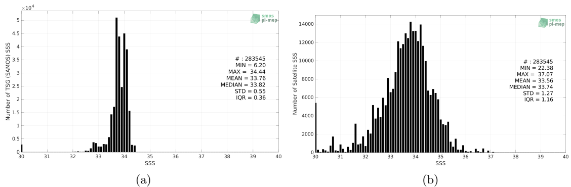
Figure 2: Histograms of SSS from TSG (SAMOS) (a) and Aquarius SSS L2 OR v5 (NASA-GSFC) (b) considering all match-up pairs per bins of 0.1 over the Southern Ocean Pi-MEP region and for the full satellite product period.
