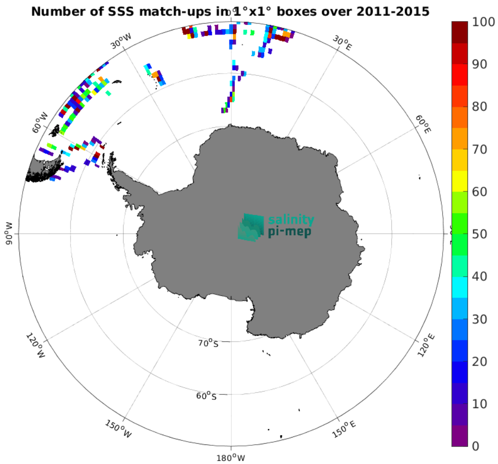
Figure 5: Number of SSS match-ups between TSG (Polarstern) SSS and the Aquarius SSS L2 OR v5 (NASA-GSFC) SSS product for the Southern Ocean Pi-MEP region over 1^\circ \times 1^\circ boxes and for the full satellite product period.
