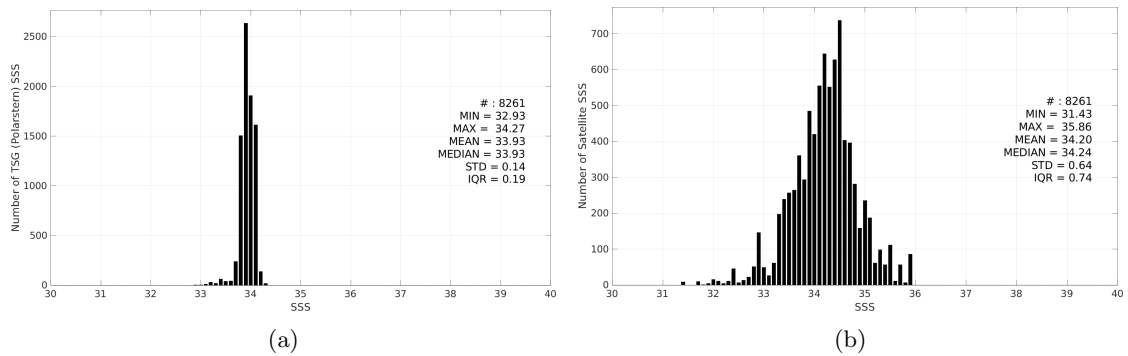
Figure 3: Histograms of SSS from TSG (Polarstern) (a) and Aquarius SSS L2 OR v5 (NASA-GSFC) (b) considering all match-up pairs per bins of 0.1 over the Southern Ocean Pi-MEP region and for the full satellite product period.
