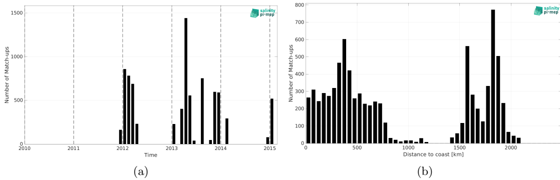
Figure 2: Number of match-ups between TSG (Polarstern) and Aquarius SSS L2 OR v5 (NASA-GSFC) SSS as a function of time (a) and as function of the distance to coast (b) over the Southern Ocean Pi-MEP region and for the full satellite product period.
