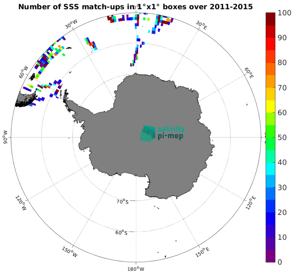
Figure 4: Number of SSS match-ups between TSG (Polarstern) SSS and the Aquarius SSS L2 OR v5 (NASA-GSFC) SSS product for the Southern Ocean Pi-MEP region over 1^{\circ} \times 1^{\circ} boxes and for the full satellite product period.
