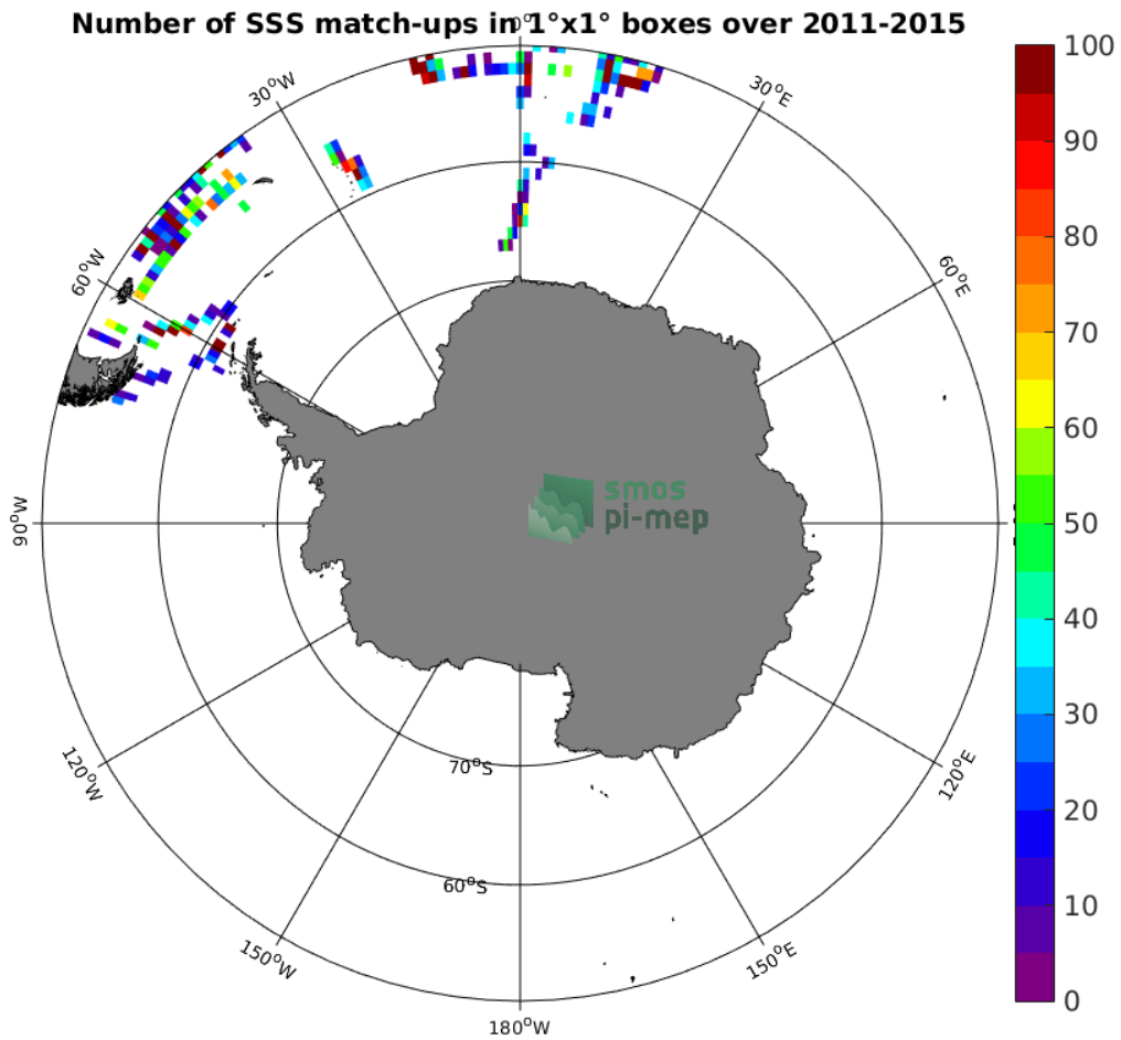
Figure 4: Number of SSS match-ups between TSG-POLARSTERN SSS and the Aquarius-L2-OR-V5 SSS product for the Southern Ocean Pi-MEP region over 1^\circ \times 1^\circ boxes and for the full satellite product period.
