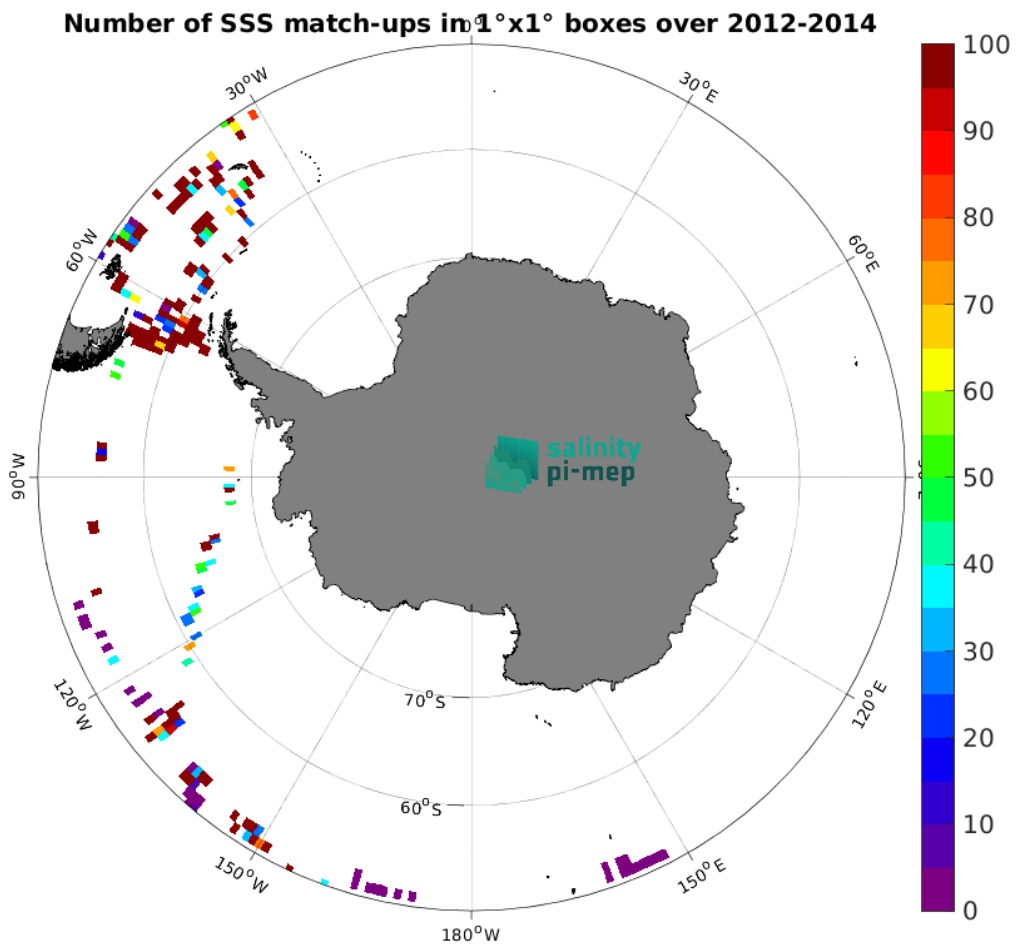
Figure 5: Number of SSS match-ups between TSG (GOSUD-Sailing-ship) SSS and the Aquarius SSS L2 OR v5 (NASA-GSFC) SSS product for the Southern Ocean Pi-MEP region over 1^\circ \times 1^\circ boxes and for the full satellite product period.
