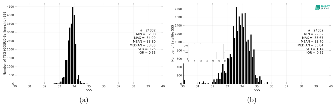
Figure 3: Histograms of SSS from TSG (GOSUD-Sailing-ship) (a) and Aquarius SSS L2 OR v5 (NASA-GSFC) (b) considering all match-up pairs per bins of 0.1 over the Southern Ocean Pi-MEP region and for the full satellite product period.
