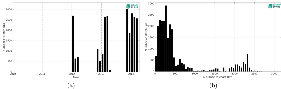
Figure 2: Number of match-ups between TSG (GOSUD-Sailing-ship) and Aquarius SSS L2 OR v5 (NASA-GSFC) SSS as a function of time (a) and as function of the distance to coast (b) over the Southern Ocean Pi-MEP region and for the full satellite product period.
