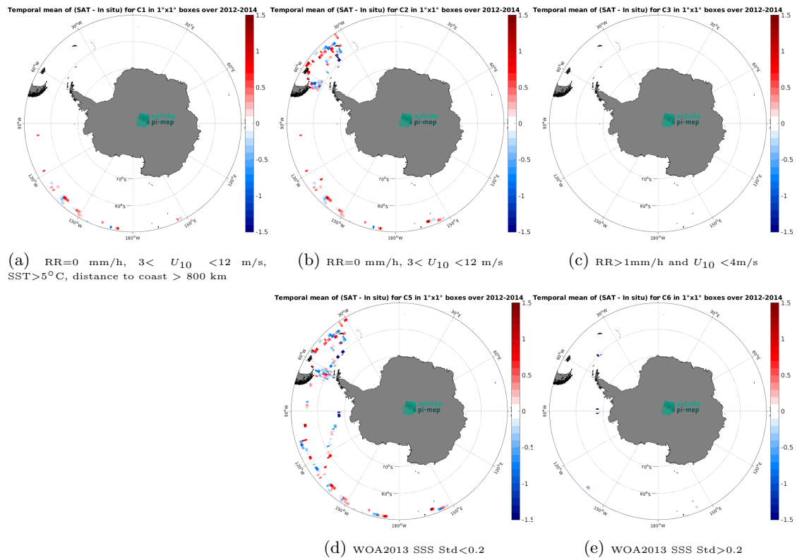
Figure 12: Temporal mean gridded over spatial boxes of size 1^\circ \times 1^\circ of \Delta\text{SSS} (Aquarius SSS L2 OR v5 (NASA-GSFC) - TSG (GOSUD-Sailing-ship)) for 5 different subdatasets corresponding to: RR=0 mm/h, 3 < U_{10} < 12 m/s, SST > 5^\circ\text{C} , distance to coast > 800 km (a), RR=0 mm/h, 3 < U_{10} < 12 m/s (b), RR > 1 mm/h and U_{10} < 4 m/s (c), WOA2013 SSS Std < 0.2 (d), WOA2013 SSS Std > 0.2 (e).
