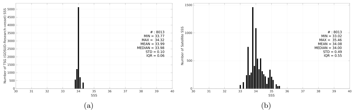
Figure 3: Histograms of SSS from TSG (GOSUD-Research-vessel) (a) and Aquarius SSS L2 OR v5 (NASA-GSFC) (b) considering all match-up pairs per bins of 0.1 over the Southern Ocean Pi-MEP region and for the full satellite product period.
