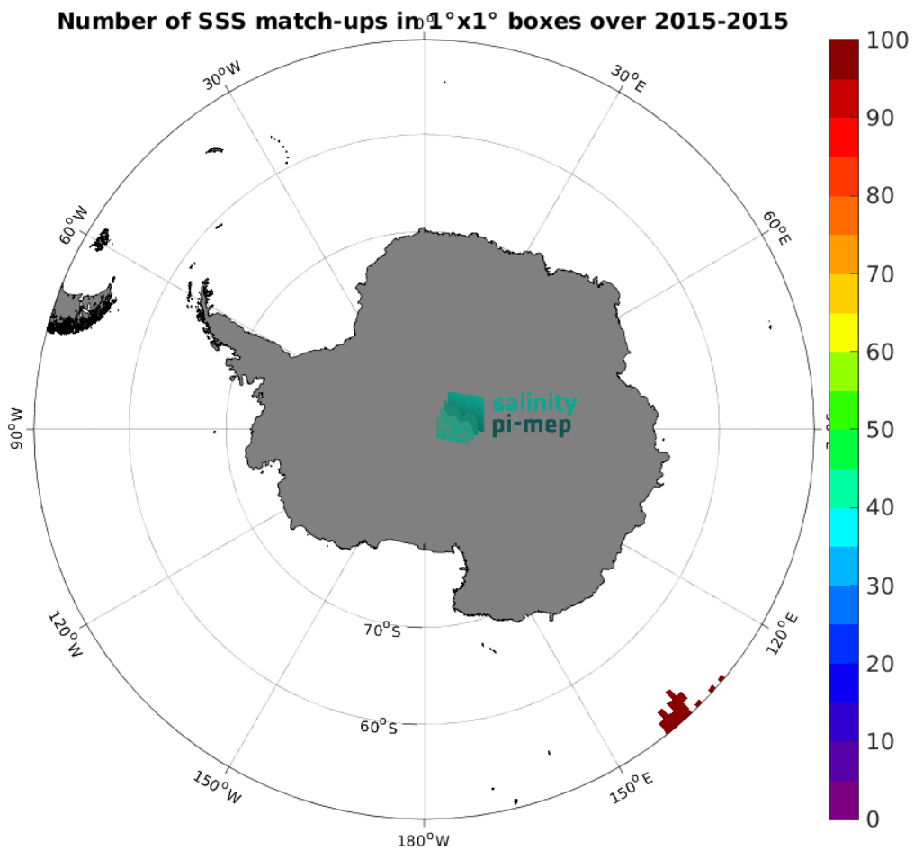
Figure 5: Number of SSS match-ups between TSG (GOSUD-Research-vessel) SSS and the Aquarius SSS L2 OR v5 (NASA-GSFC) SSS product for the Southern Ocean Pi-MEP region over 1^\circ \times 1^\circ boxes and for the full satellite product period.
