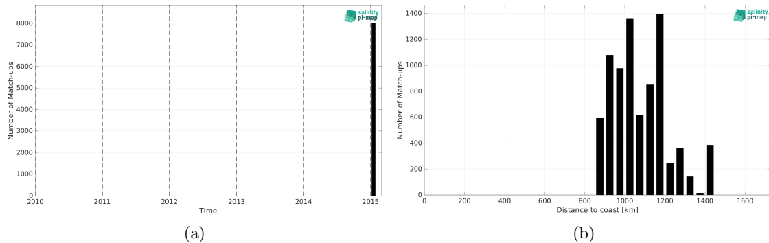
Figure 2: Number of match-ups between TSG (GOSUD-Research-vessel) and Aquarius SSS L2 OR v5 (NASA-GSFC) SSS as a function of time (a) and as function of the distance to coast (b) over the Southern Ocean Pi-MEP region and for the full satellite product period.
