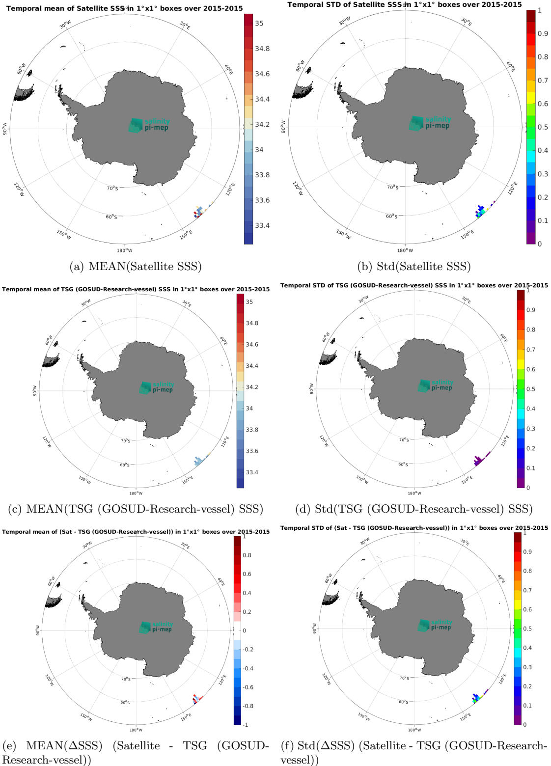
Figure 7: Temporal mean (left) and Std (right) of SSS from Aquarius SSS L2 OR v5 (NASA-GSFC) (top), TSG (GOSUD-Research-vessel) (middle), and of \Delta SSS (Satellite - TSG (GOSUD-Research-vessel)). Only match-up pairs are used to generate these maps.
