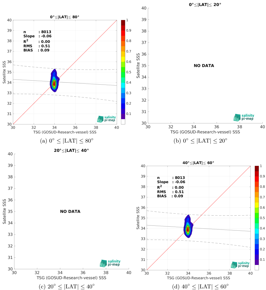
Figure 10: Contour maps of the concentration of Aquarius SSS L2 OR v5 (NASA-GSFC) SSS (y-axis) versus TSG (GOSUD-Research-vessel) SSS (x-axis) at match-up pairs for different latitude bands. For each plot, the red line shows x=y . The black thin and dashed lines indicate a linear fit through the data cloud and the \pm 95\% confidence levels, respectively. The number match-up pairs n , the slope and R^2 coefficient of the linear fit, the root mean square (RMS) and the mean bias between satellite and in situ data are indicated for each latitude band in each plots.
