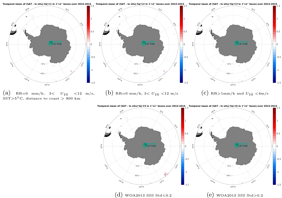
Figure 14: Temporal mean gridded over spatial boxes of size 1^\circ \times 1^\circ of \Delta\text{SSS} (Aquarius SSS L2 OR v5 (NASA-GSFC) - TSG (GOSUD-Research-vessel)) for 5 different subdatasets corresponding to:RR=0 mm/h, 3 < U_{10} < 12 m/s, SST>5°C, distance to coast > 800 km (a), RR=0 mm/h, 3 < U_{10} < 12 m/s (b), RR>1mm/h and U_{10} < 4 m/s (c), WOA2013 SSS Std<0.2 (d), WOA2013 SSS Std>0.2 (e).
