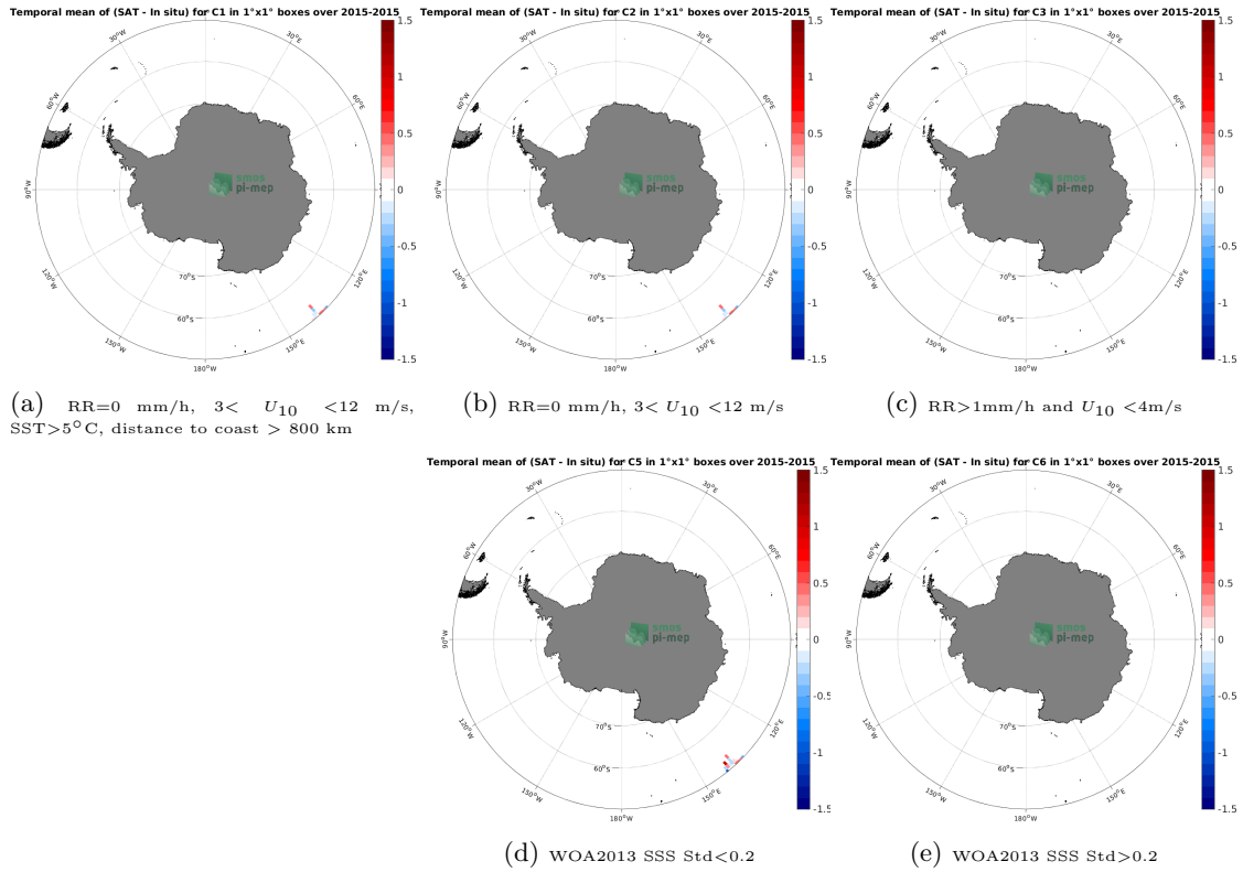
Figure 12: Temporal mean gridded over spatial boxes of size 1^{\circ} \times 1^{\circ} of \Delta SSS (Aquarius SSS L2 OR v5 (NASA-GSFC) - TSG (GOSUD-Research-vessel)) for 5 different subdatasets corresponding to: RR=0 mm/h, 3 < U_{10} < 12 m/s, SST > 5°C, distance to coast > 800 km (a), RR=0 mm/h, 3 < U_{10} < 12 m/s (b), RR > 1mm/h and U_{10} < 4 m/s (c), WOA2013 SSS Std < 0.2 (d), WOA2013 SSS Std > 0.2 (e).
