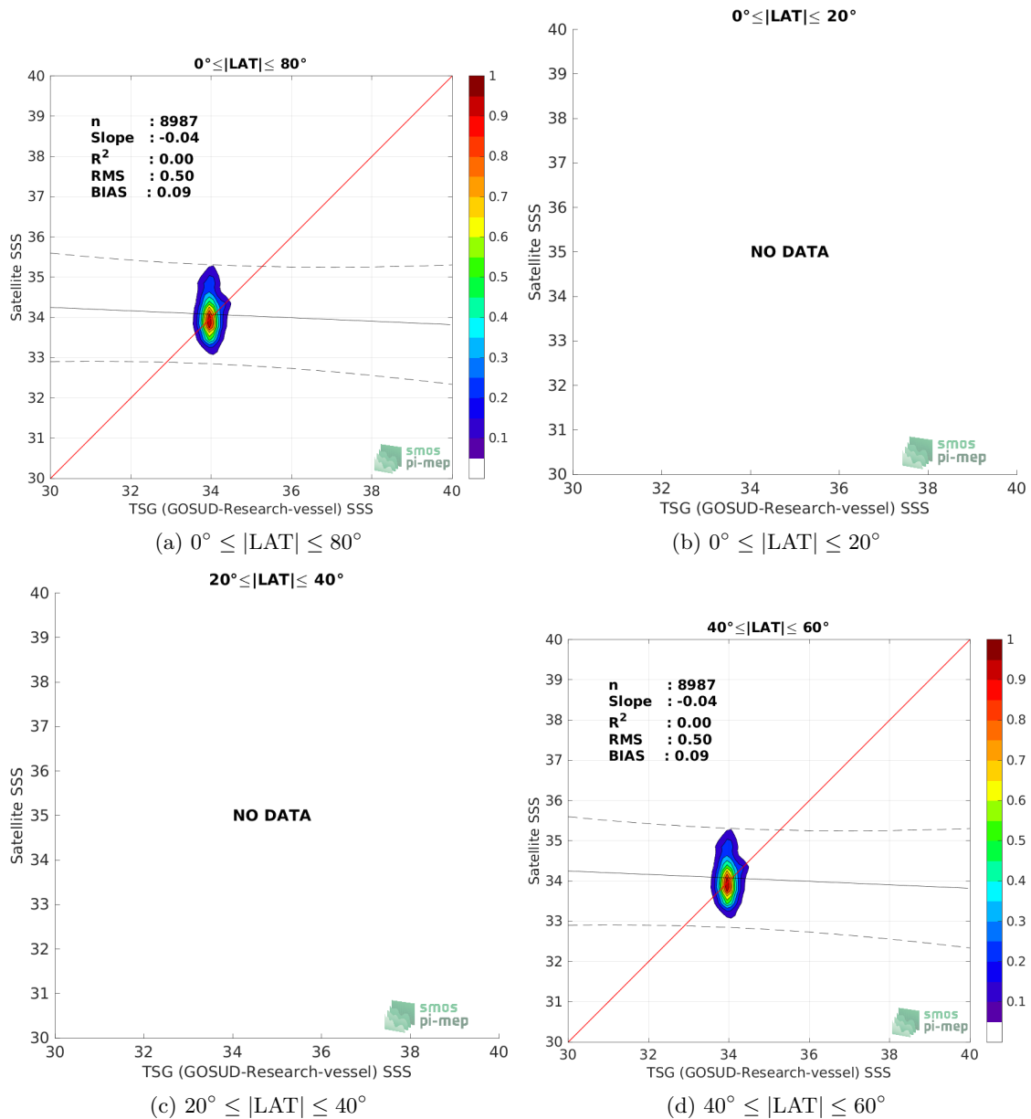
Figure 9: Contour maps of the concentration of Aquarius SSS L2 OR v5 (NASA-GSFC) SSS (y-axis) versus TSG (GOSUD-Research-vessel) SSS (x-axis) at match-up pairs for different latitude bands. For each plot, the red line shows x=y . The black thin and dashed lines indicate a linear fit through the data cloud and the \pm 95\% confidence levels, respectively. The number match-up pairs n , the slope and R^2 coefficient of the linear fit, the root mean square (RMS) and the mean bias between satellite and in situ data are indicated for each latitude band in each plots.
