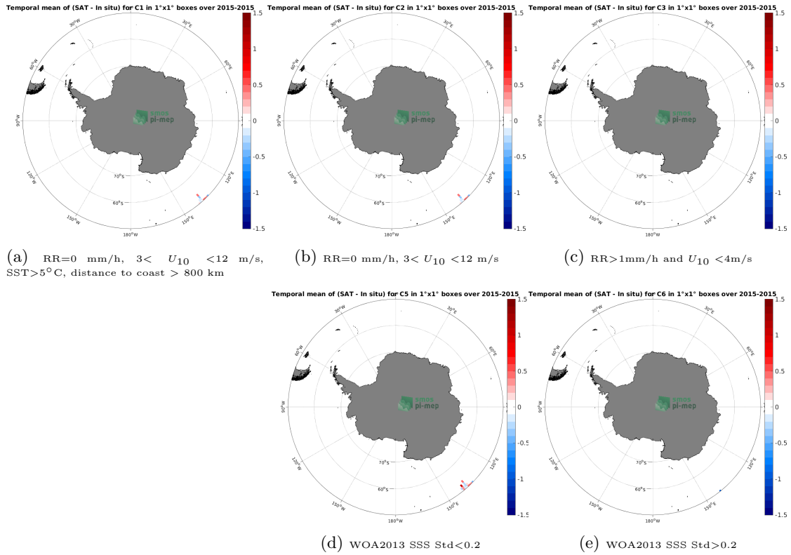
Figure 12: Temporal mean gridded over spatial boxes of size 1^\circ \times 1^\circ of \Delta SSS (Aquarius SSS L2 OR v5 (NASA-GSFC) - TSG (GOSUD-Research-vessel)) for 5 different subdatasets corresponding to: RR=0 mm/h, 3 < U_{10} < 12 m/s, SST>5°C, distance to coast > 800 km (a), RR=0 mm/h, 3 < U_{10} < 12 m/s (b), RR>1mm/h and U_{10} < 4 m/s (c), WOA2013 SSS Std<0.2 (d), WOA2013 SSS Std>0.2 (e).
