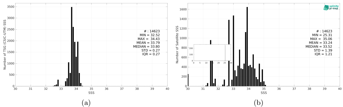
Figure 3: Histograms of SSS from TSG (CSIC-UTM) (a) and Aquarius SSS L2 OR v5 (NASA-GSFC) (b) considering all match-up pairs per bins of 0.1 over the Southern Ocean Pi-MEP region and for the full satellite product period.
