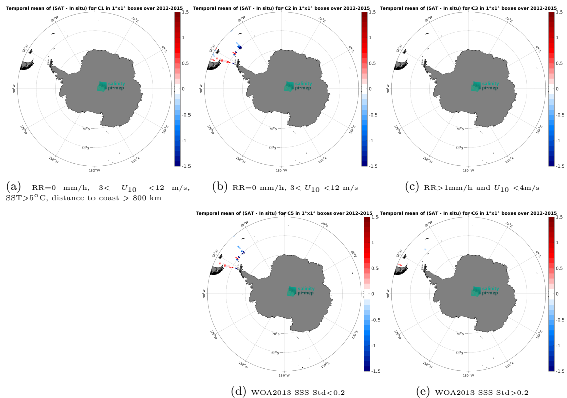
Figure 14: Temporal mean gridded over spatial boxes of size 1^\circ \times 1^\circ of \Delta\text{SSS} (Aquarius SSS L2 OR v5 (NASA-GSFC) - TSG (CSIC-UTM)) for 5 different subdatasets corresponding to: RR=0 mm/h, 3 < U_{10} < 12 m/s, SST > 5°C, distance to coast > 800 km (a), RR=0 mm/h, 3 < U_{10} < 12 m/s (b), RR > 1mm/h and U_{10} < 4 m/s (c), WOA2013 SSS Std < 0.2 (d), WOA2013 SSS Std > 0.2 (e).
