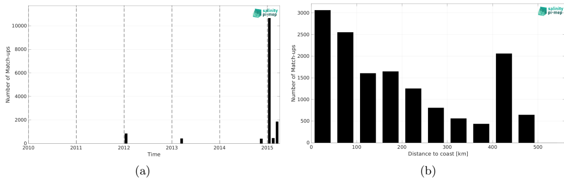
Figure 2: Number of match-ups between TSG (CSIC-UTM) and Aquarius SSS L2 OR v5 (NASA-GSFC) SSS as a function of time (a) and as function of the distance to coast (b) over the Southern Ocean Pi-MEP region and for the full satellite product period.
