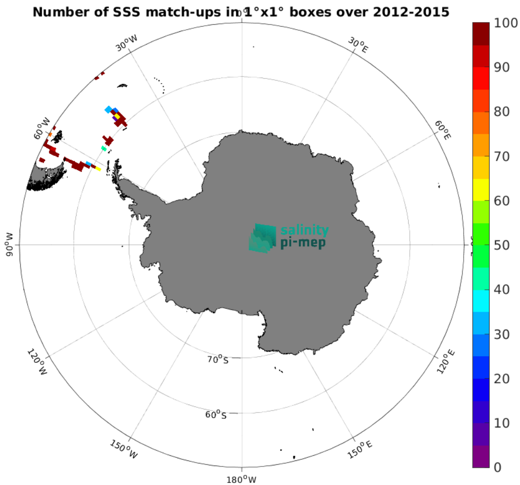
Figure 5: Number of SSS match-ups between TSG (CSIC-UTM) SSS and the Aquarius SSS L2 OR v5 (NASA-GSFC) SSS product for the Southern Ocean Pi-MEP region over 1^\circ \times 1^\circ boxes and for the full satellite product period.
